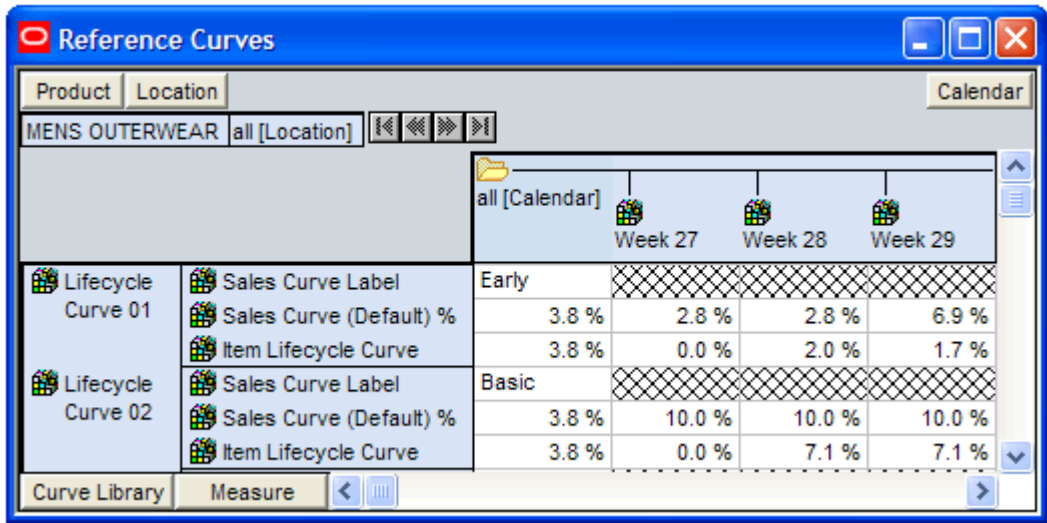
Figure 7–7 Reference Curves Worksheet
