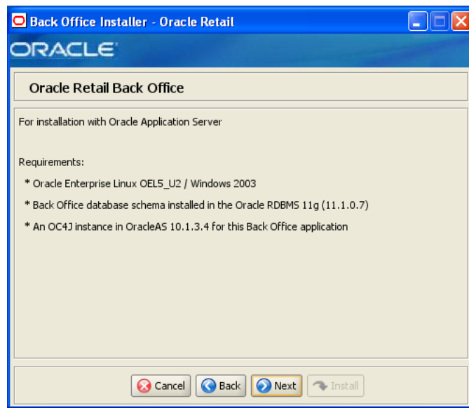
Figure B–2 Requirements
