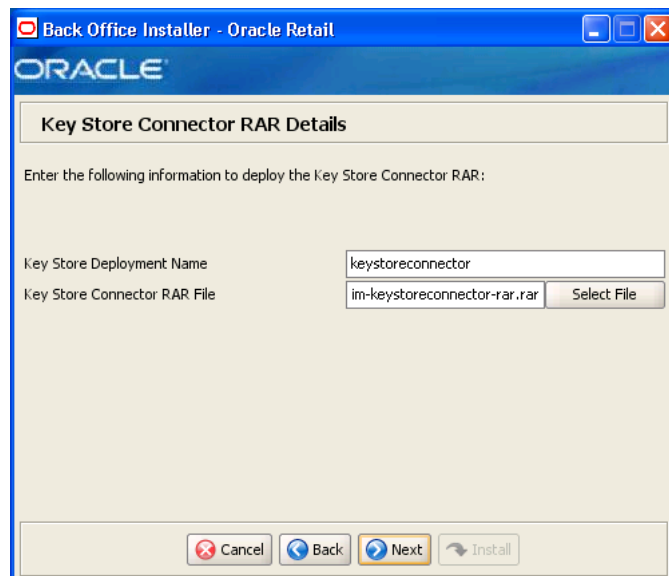
Figure C–19 Key Store Connector RAR Details
