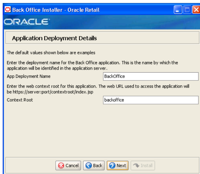
Figure C–31 Application Deployment Details
