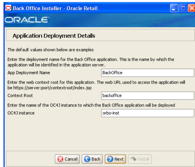
Figure B–28 Application Deployment Details
