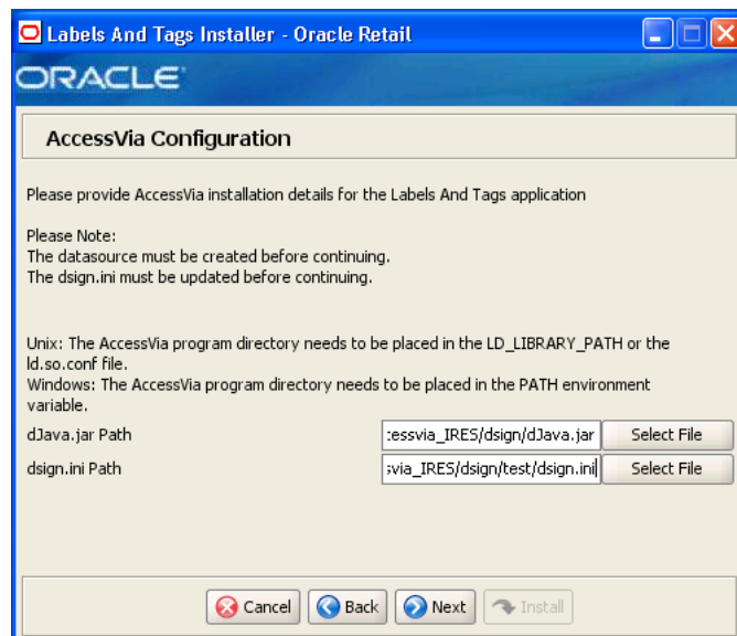
Figure C-22 Access Via Configuration
