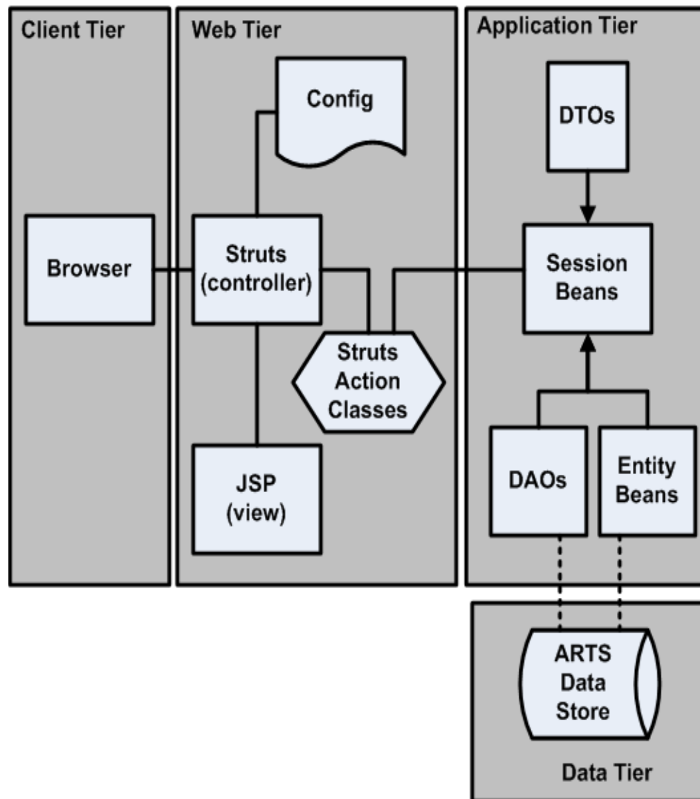
Figure 2–1 High-Level Architecture
