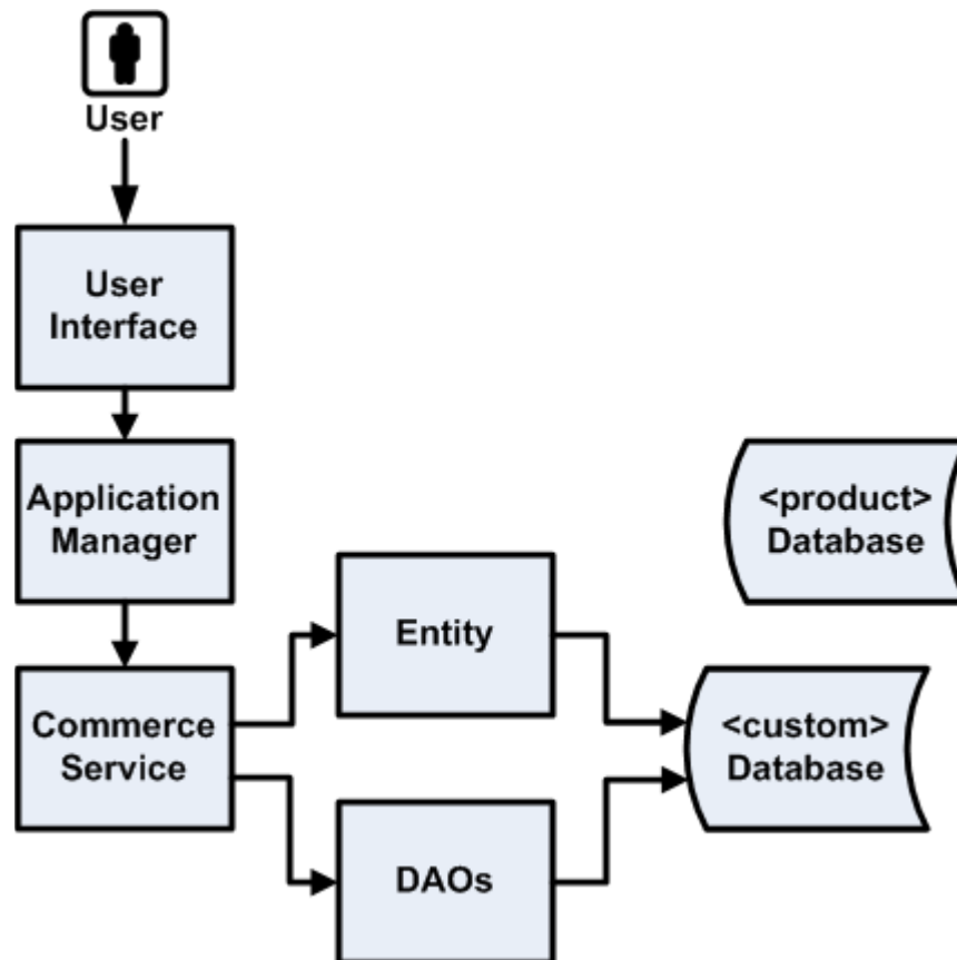
Figure 7–4 Accessing Data from a Different Database
