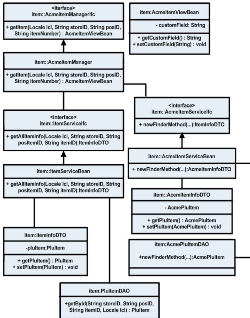
Figure 7-13 Extension with Composition: Class Diagram -- DAO
