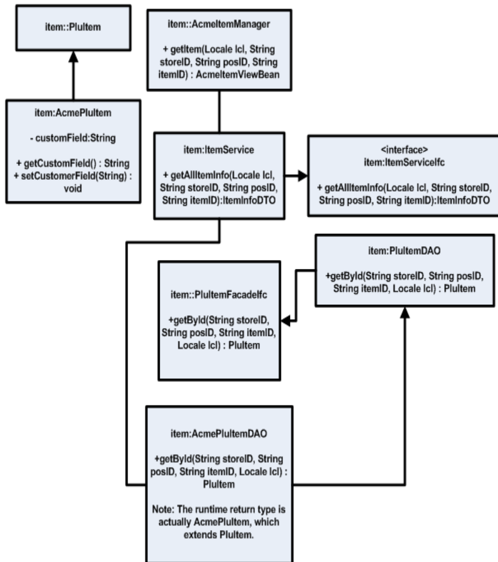
Figure 7-17 Data Extension Through Composition: Class Diagram -- DAO
