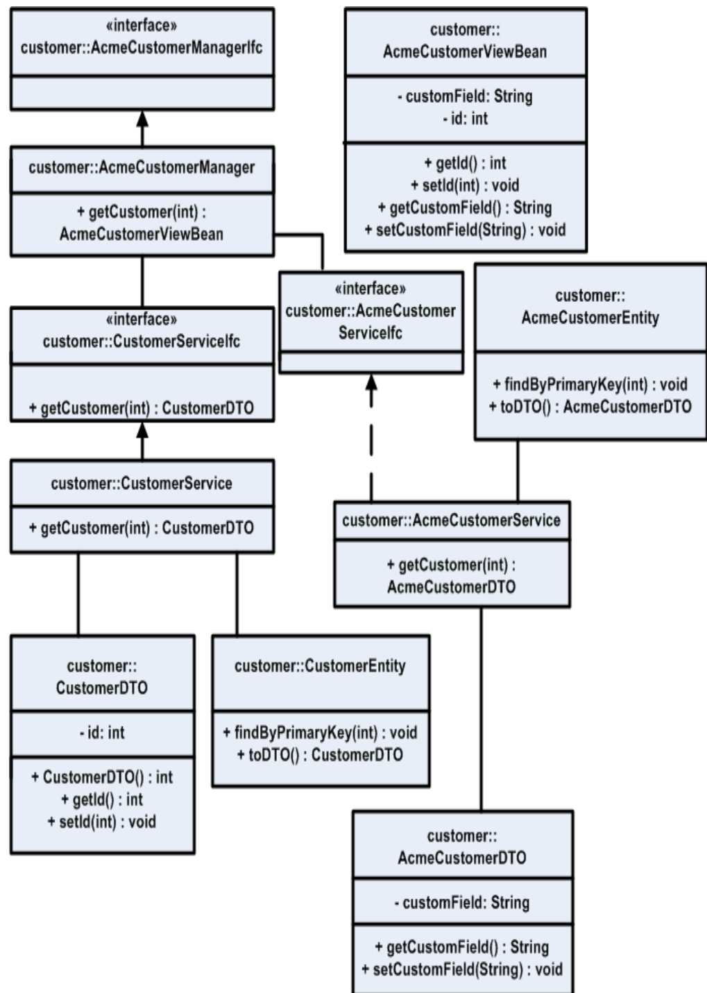
Figure 7-12 Extension with Composition: Class Diagram -- Entity Bean
