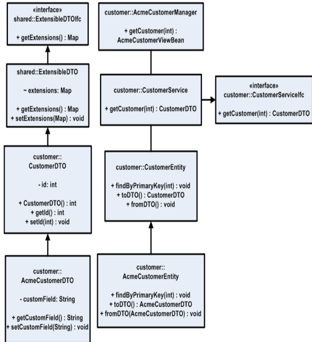
Figure 7-16 Data Extension Through Composition: Class Diagram -- Entity Bean
