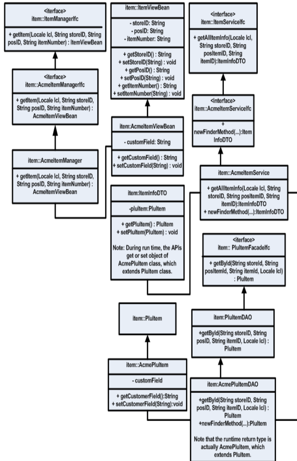
Figure 7-10 Extension with Inheritance: Class Diagram -- DAO
