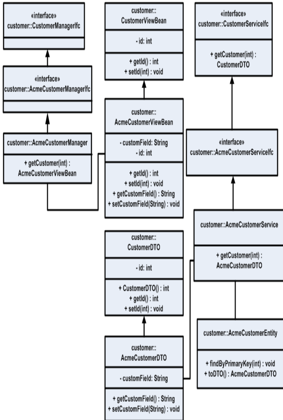
Figure 7–9 Extension with Inheritance: Class Diagram -- Entity Bean
