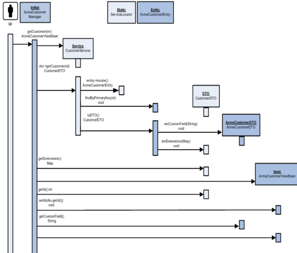
Figure 7–15 Data Extension through Composition
