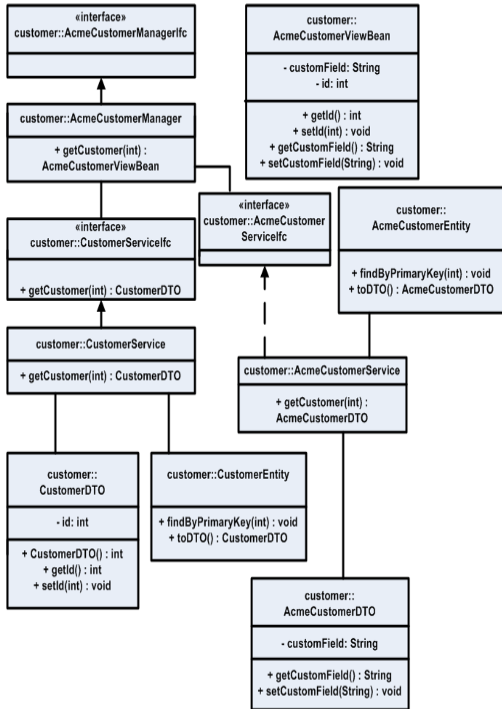
Figure 7-12 Extension with Composition: Class Diagram—Entity Bean
