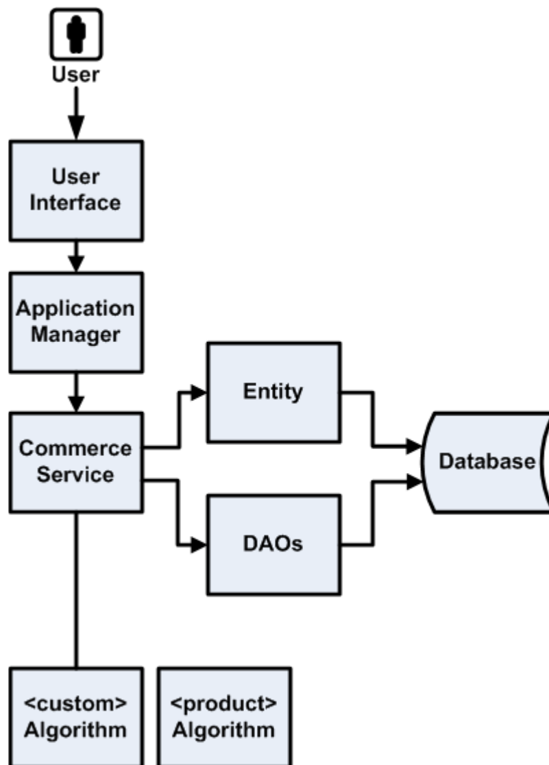
Figure 7–6 Application Layers
