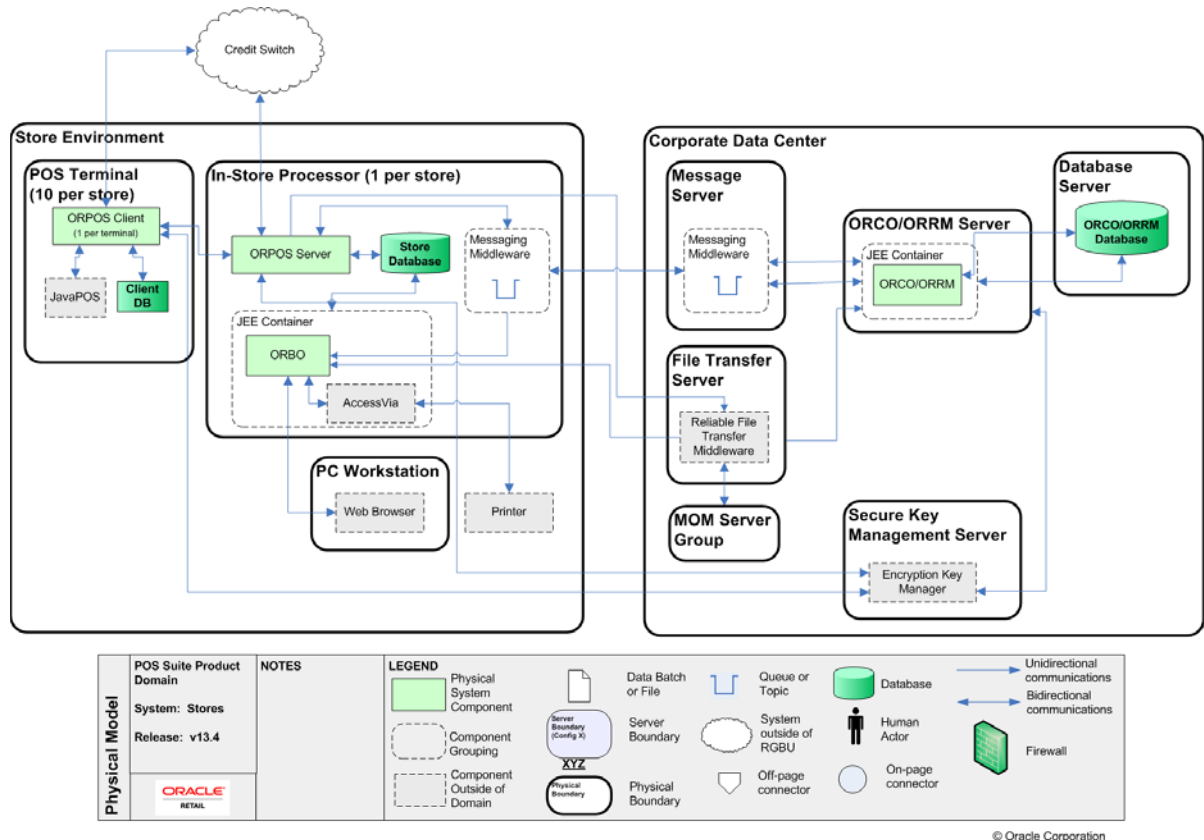
Figure 1-1 Oracle Retail POS Suite Security Features
