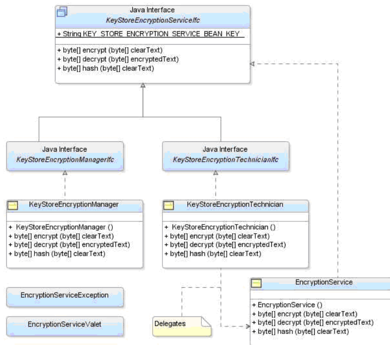
Figure 1–3 Java Interface
