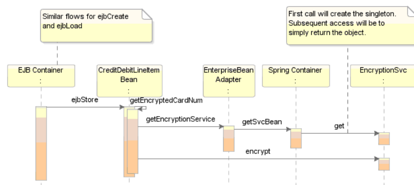
Figure 1–6 EJB Flow
