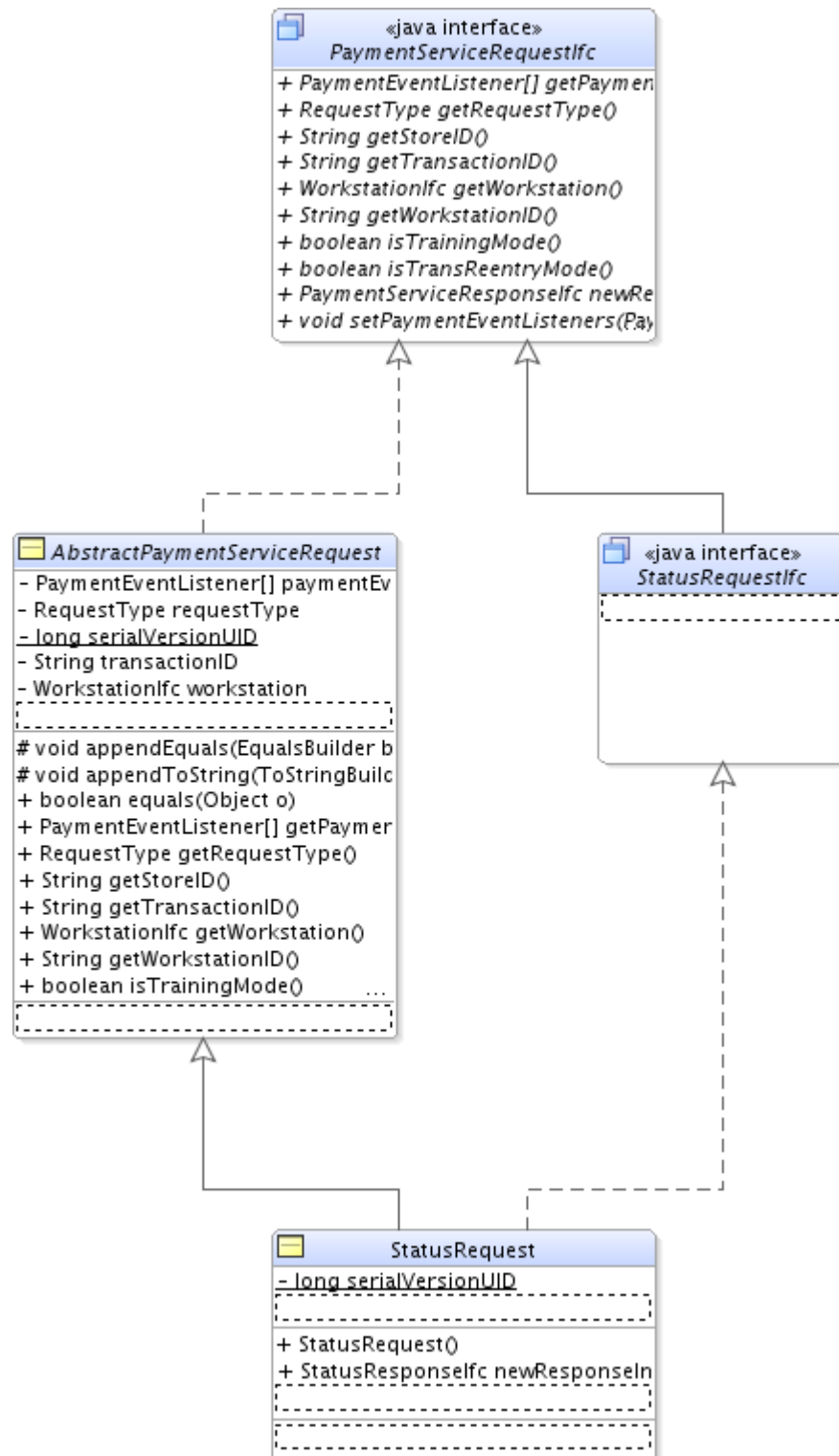
Figure 12–7 StatusRequest Class
