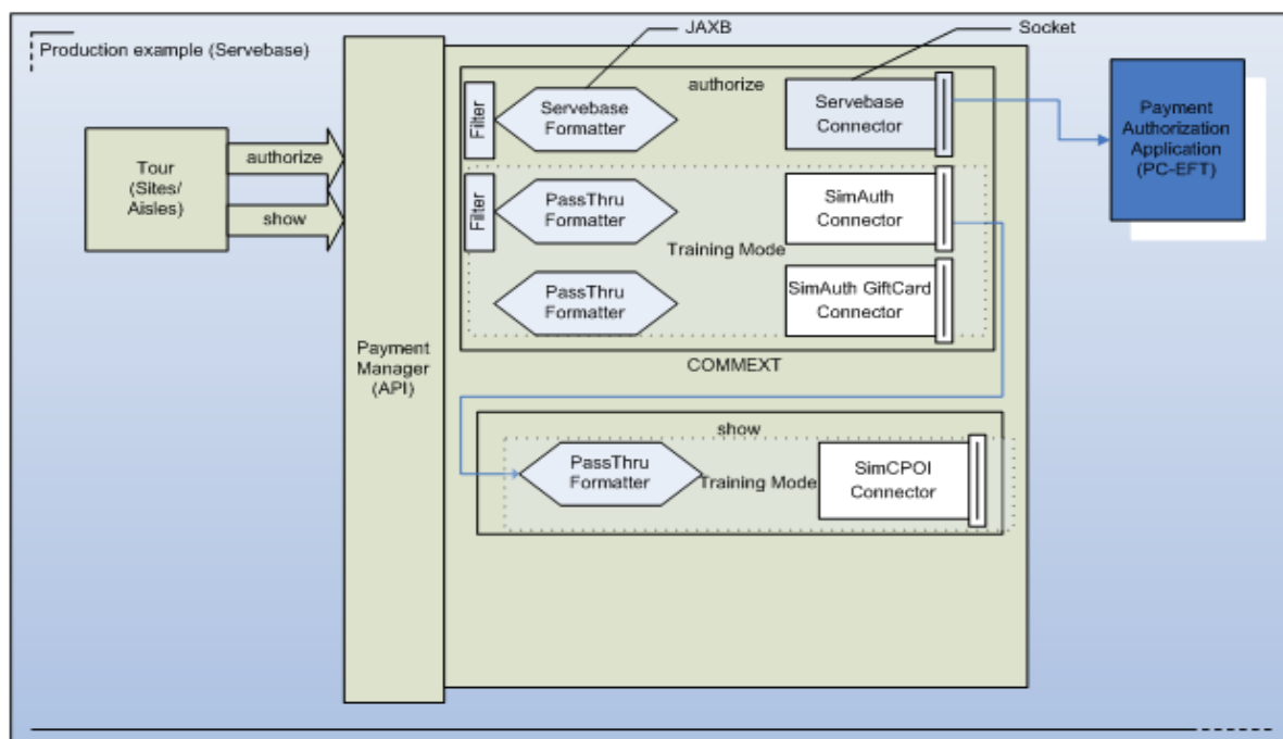
Figure 12-14 APF Flow Diagram
