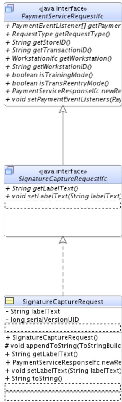
Figure 12–5 SignatureCaptureRequest Class
