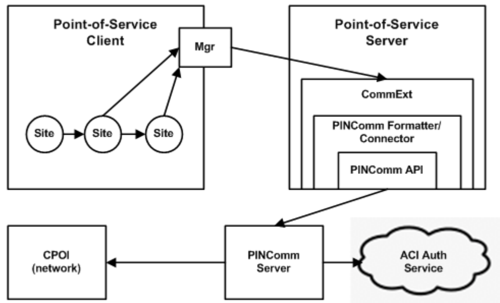
Figure 12–9 PinComm Topology
