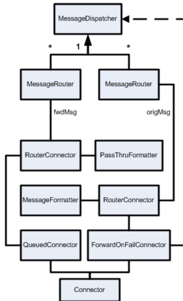
Figure 13–6 Attempt, Store and Forward on Failure in COMNEXT
