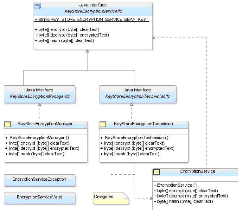
Figure 1–3 Java Interface
