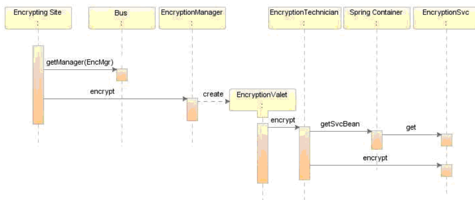
Figure 1–8 POS Flow
