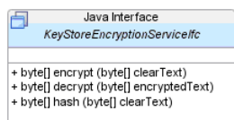
Figure 3–1 KeyStoreEncryptionServiceIcfc Class
