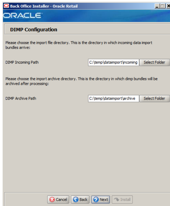
Figure A-11 DIMP Configuration
