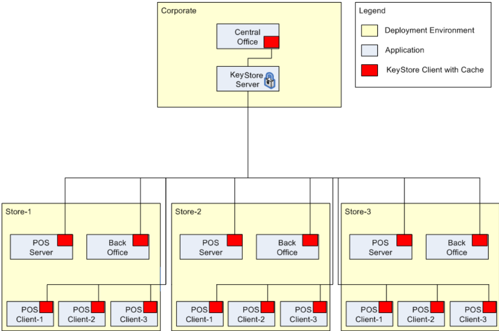
Figure 1-2 Deployment Model
