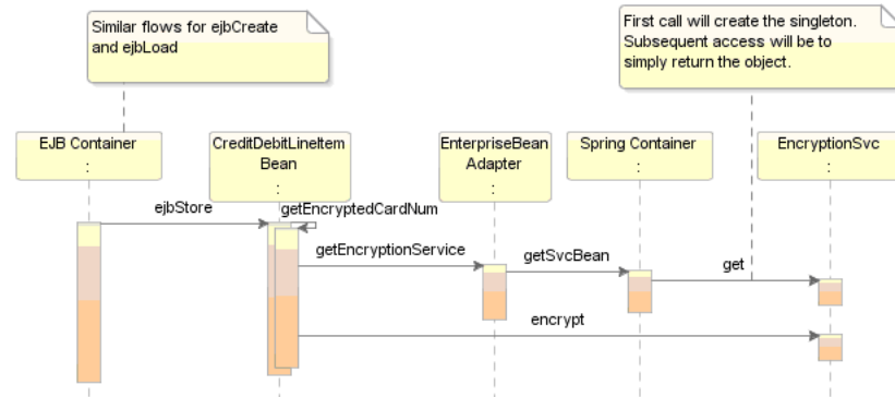
Figure 1-6 EJB Flow
