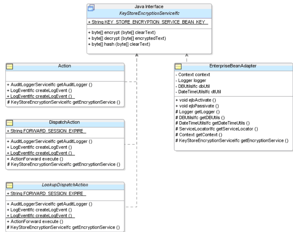
Figure 1–4 J2EE Class Updates
