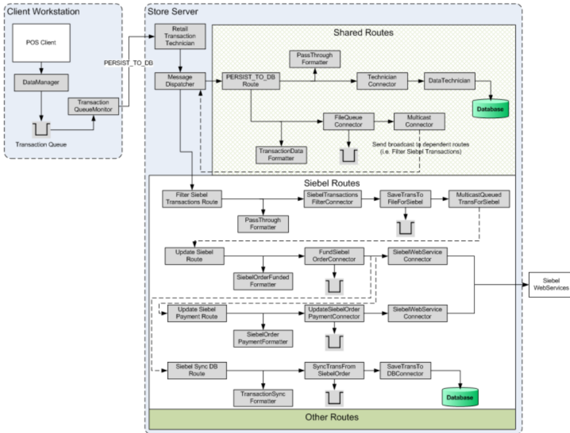
Figure 3–3 Update External Order Routes
