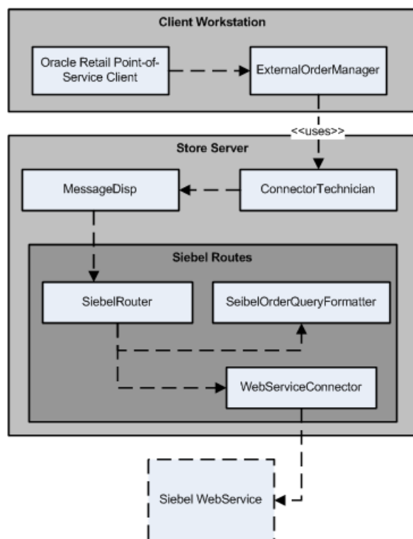
Figure 3–1 External Order Interaction
