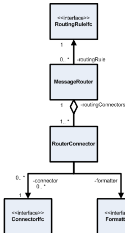
Figure 2-2 Message Routing Details
