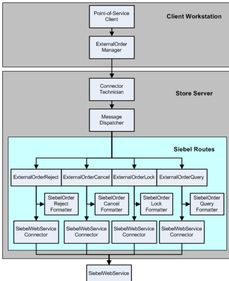
Figure 3–2 Query External Order Routes
