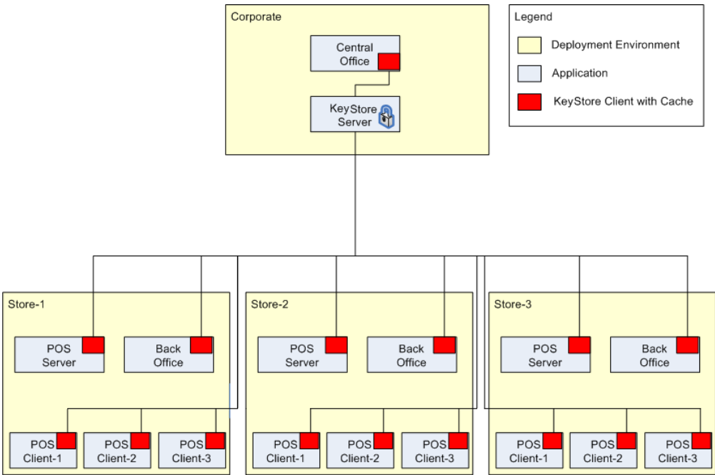
Figure 1-2 Deployment Model
