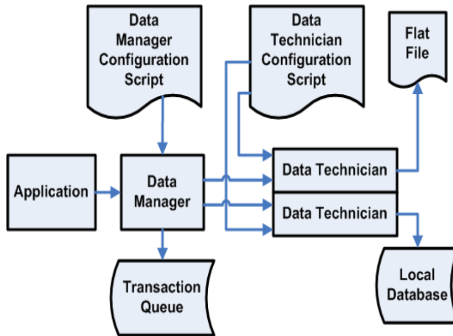
Figure 2–6 Data Persistence Framework
