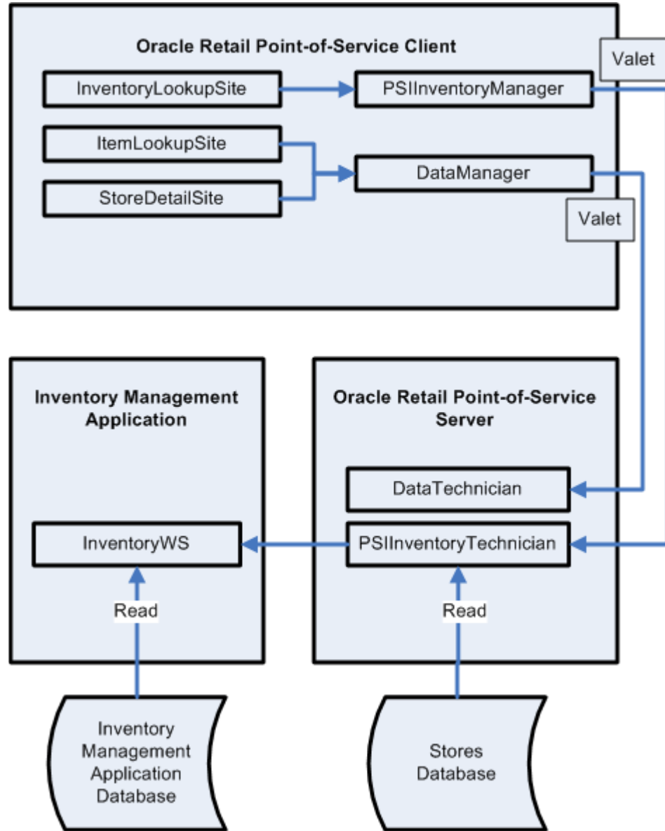
Figure F–1 High-Level Model for Oracle Retail Point-of-Service to an Inventory Management Application Integration
