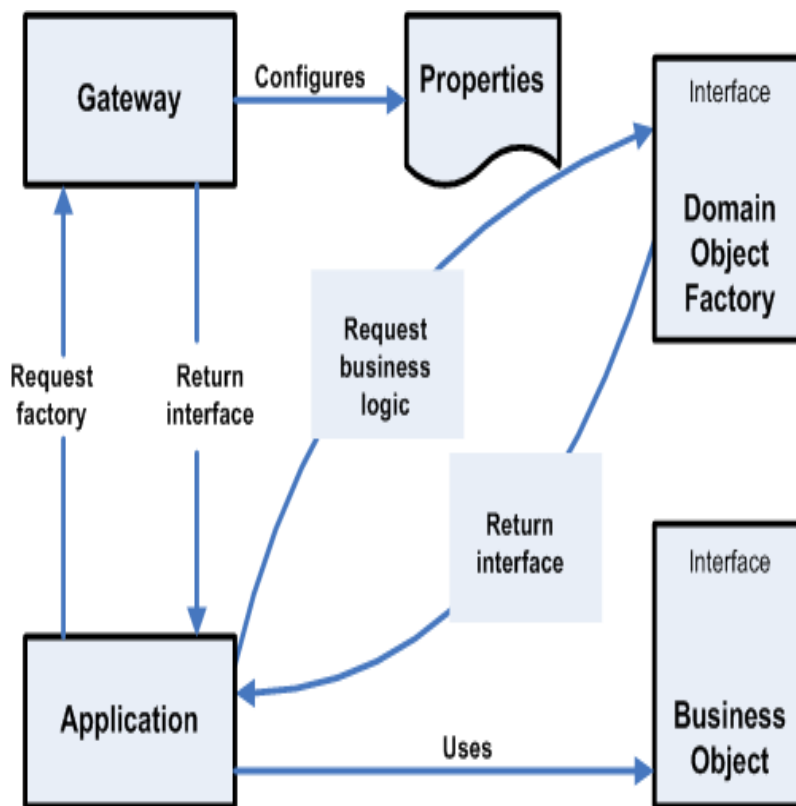
Figure 2–5 Business Object Framework
