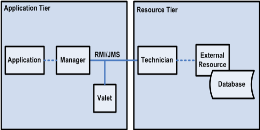
Figure 2–3 Manager/Technician Framework
