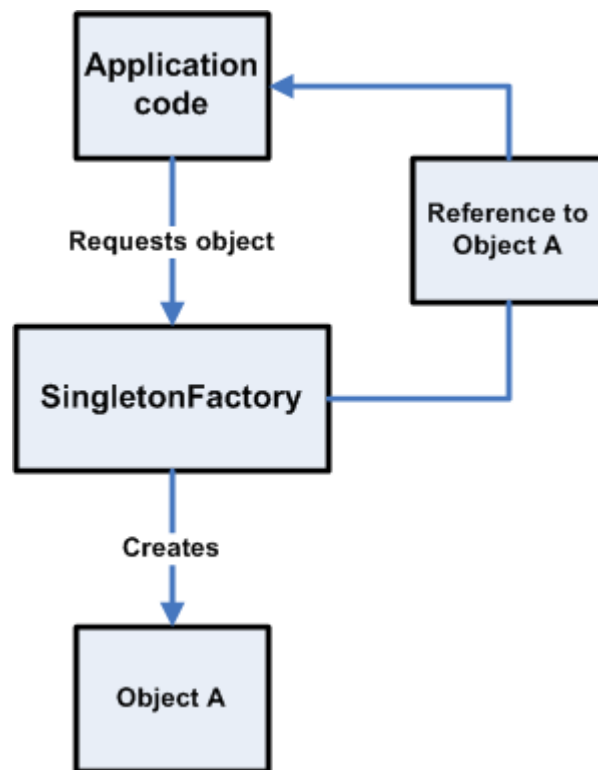
Figure 2–10 Singleton Pattern
