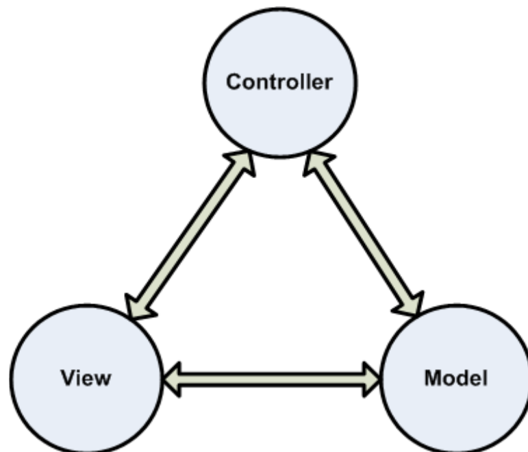
Figure 2–7 MVC Pattern
