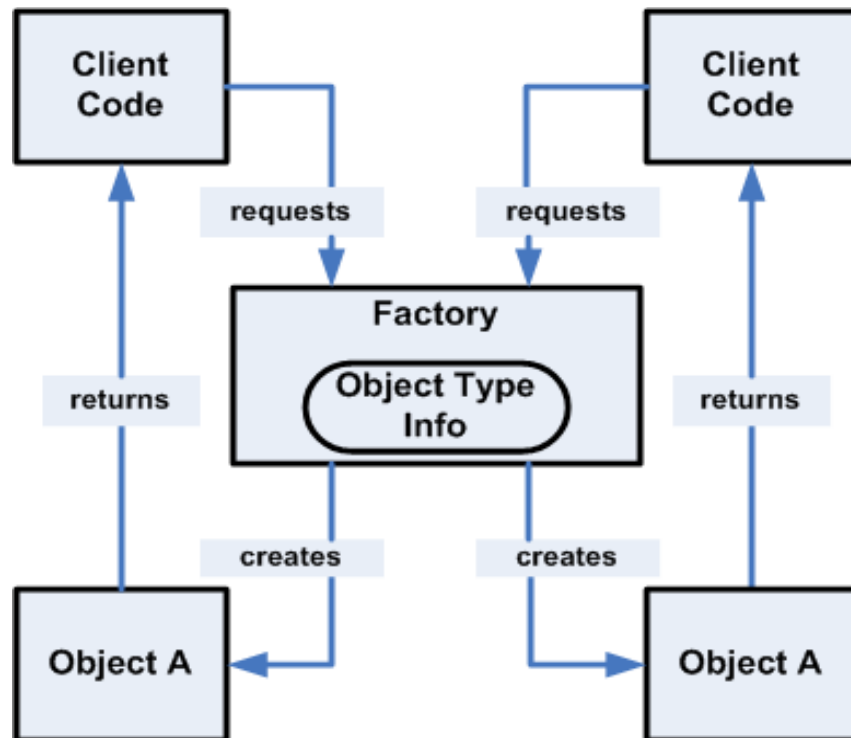
Figure 2–8 Factory Pattern
