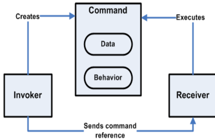
Figure 2–9 Command Pattern
