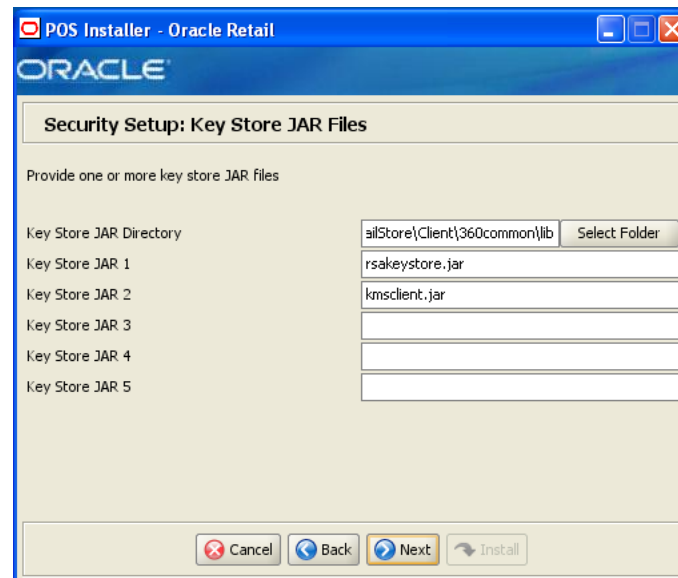
Figure B–26 Security Setup: Key Store JAR Files for RSA Key Manager 3.1
