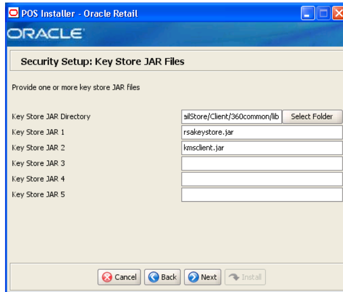
Figure D–27 Security Setup: Key Store JAR Files for RSA Key Manager 3.1
