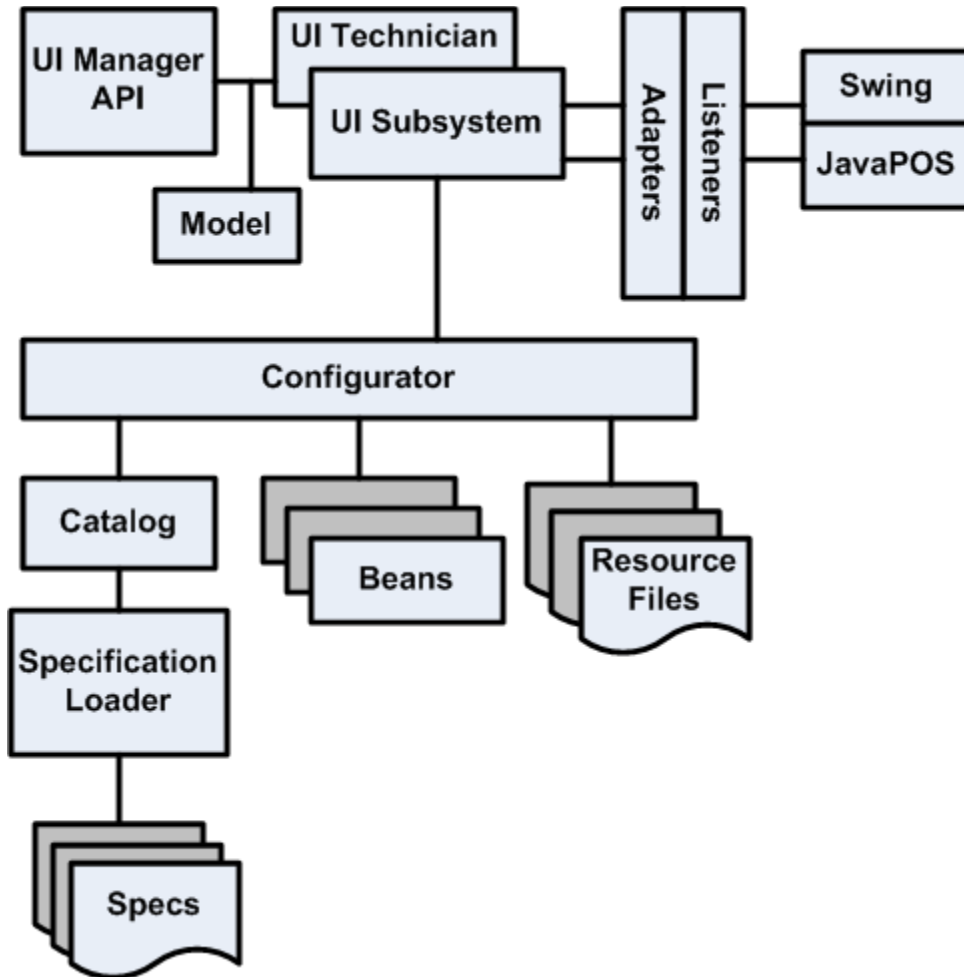
Figure 9-2 UI Framework
