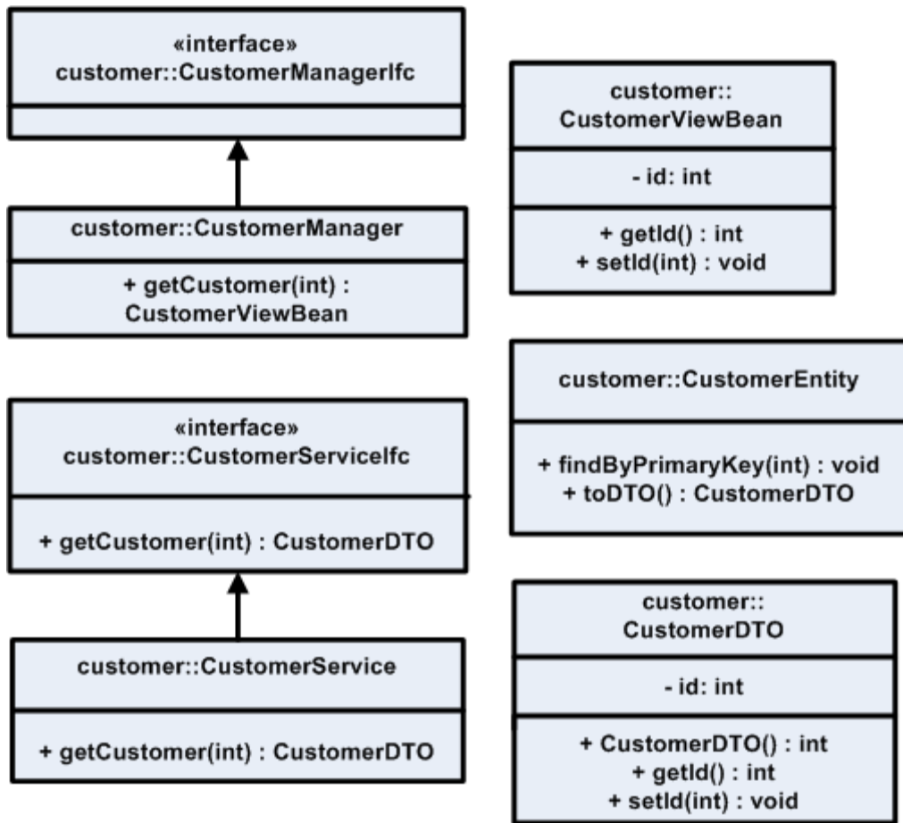
Figure 6-7 Sample Classes for Extension—Entity Bean
