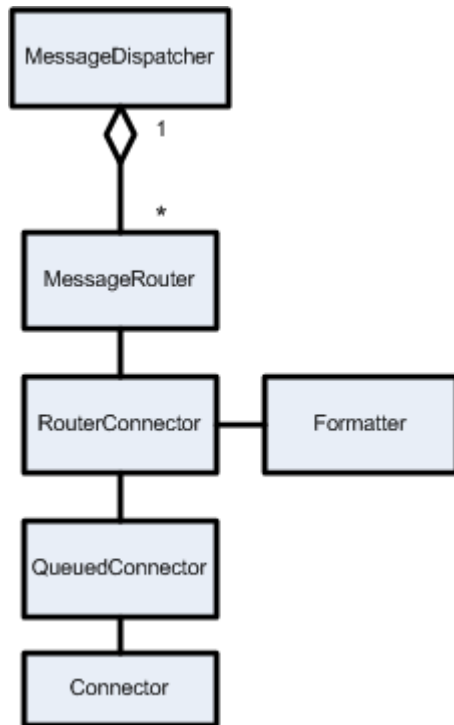
Figure 13–5 Store and Forward Operations in COMMEXT
