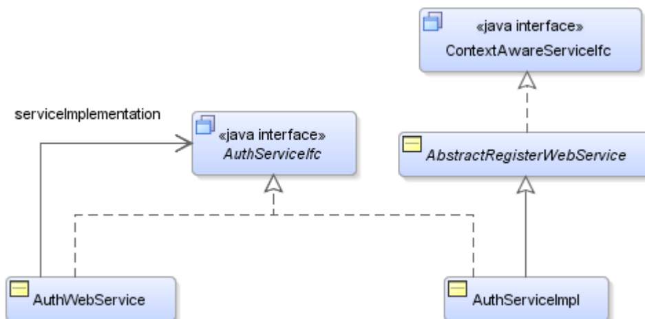
Figure 4-1 Service Framework
