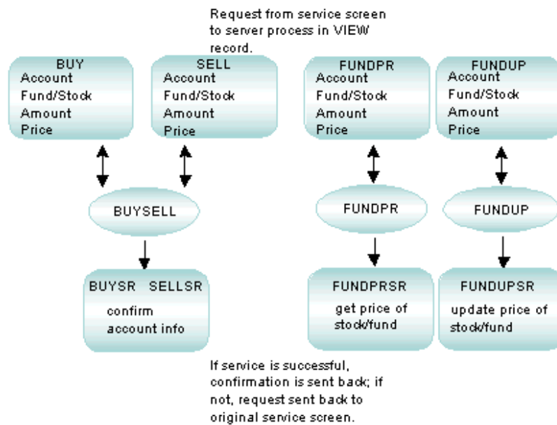
Figure 5-1 STOCKAPP Requests
