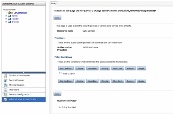
Figure 5-19 Administrative Access Control Tab
