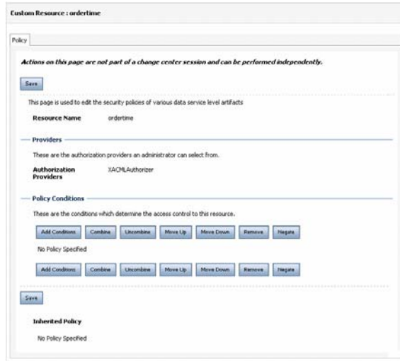
Figure 5-18 Creating Runtime Security Policy for a User-Defined Security Resource
