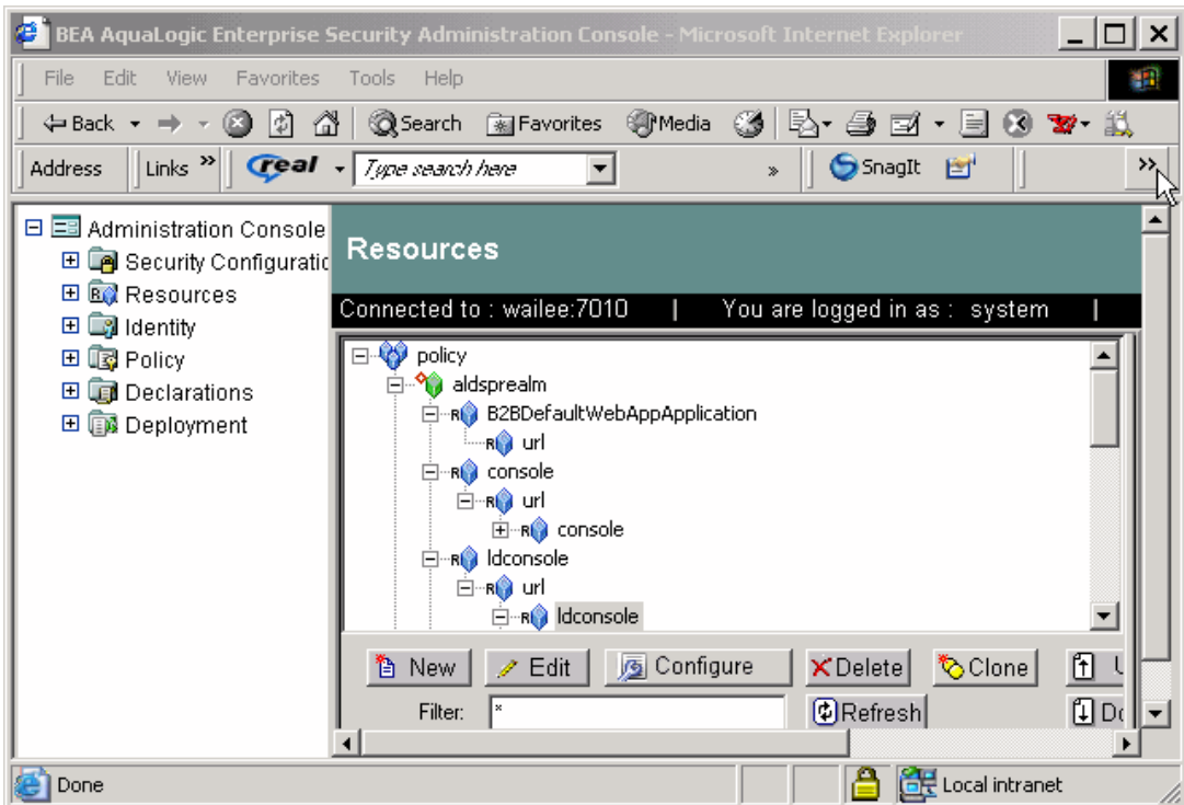
Figure 3-3 Administration Console
