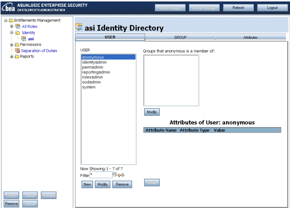
Figure 5-5 Users Tab
