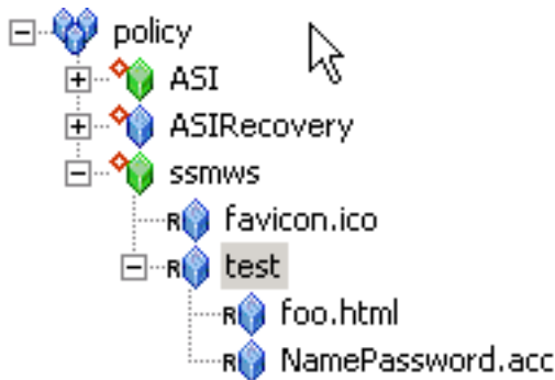
Figure 3-5 Defined Resources
