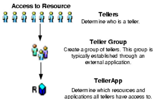
Figure 2-1 Resource Mapping
