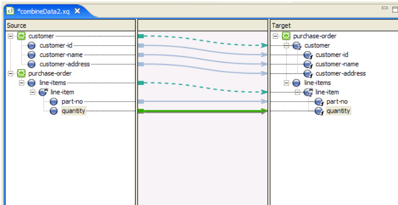
Figure 3-2 Data Transformation in Design View
