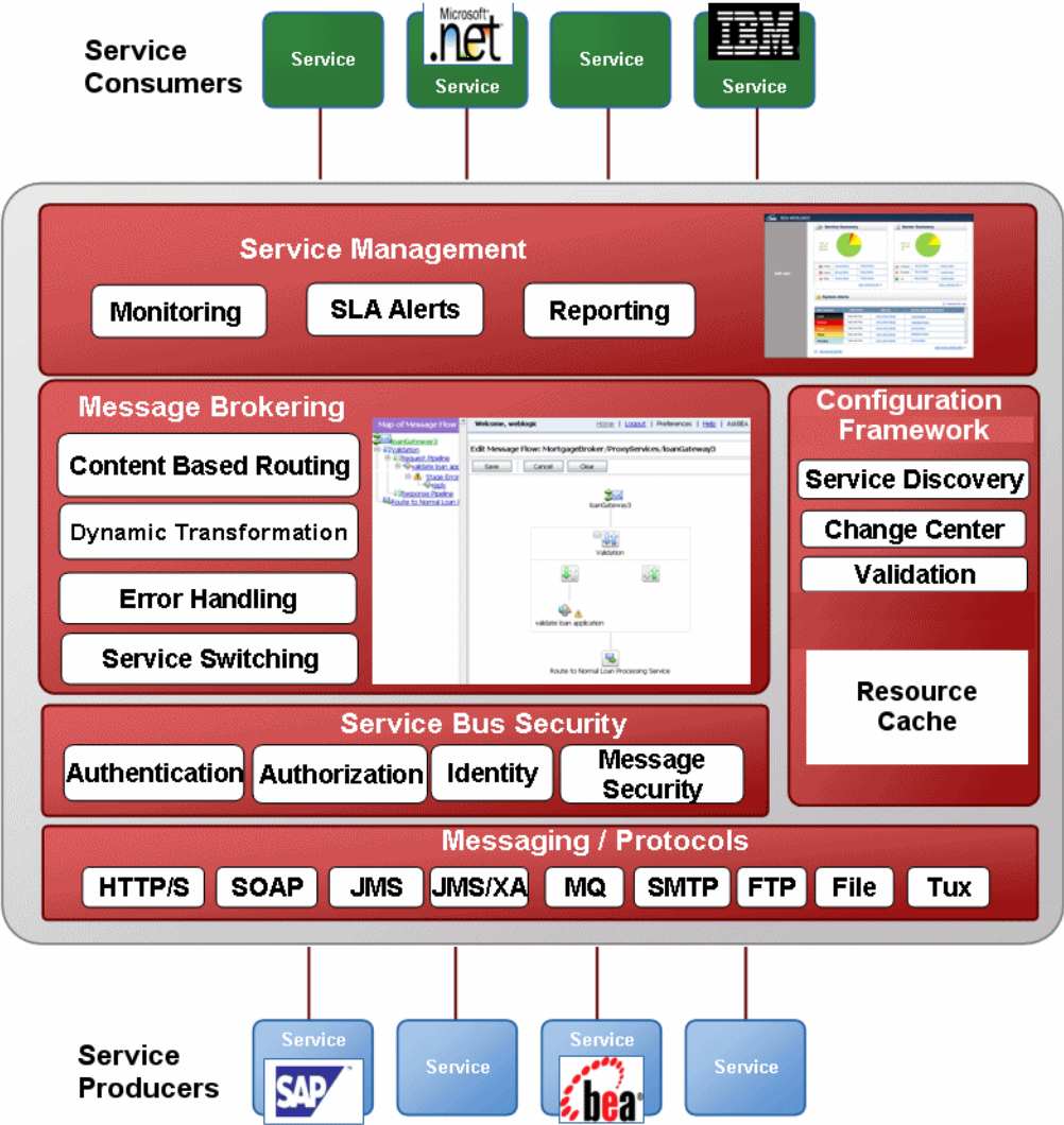
Figure 2-2 AquaLogic Service Bus High-Level Architecture
