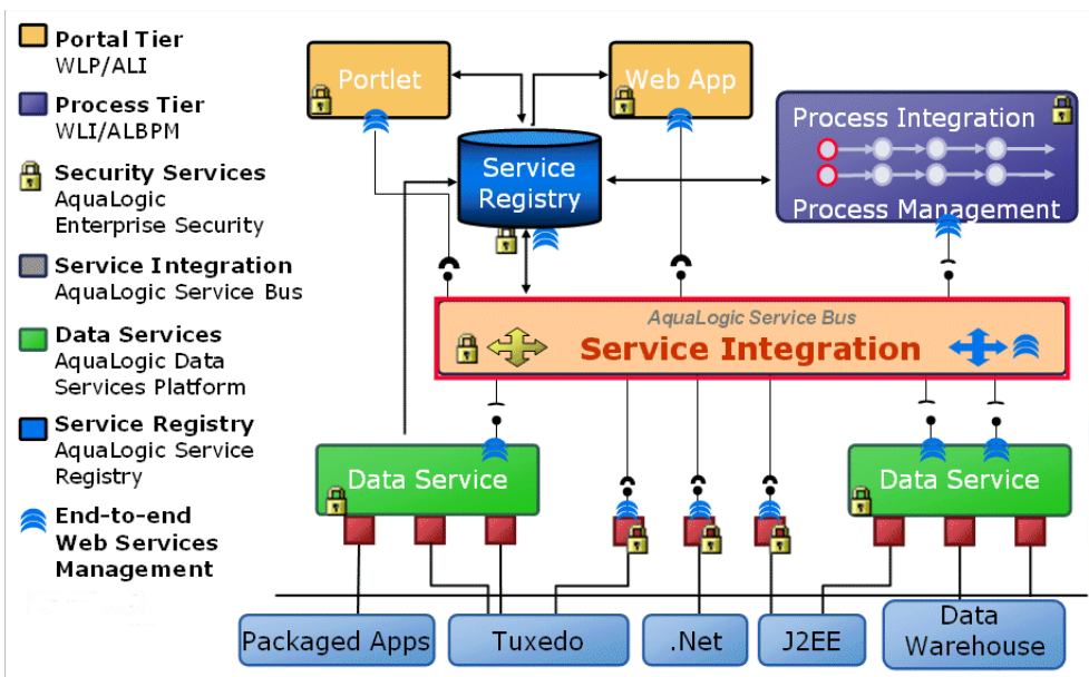
Figure 1-9 AquaLogic Service Bus Significance in SOA Architecture
