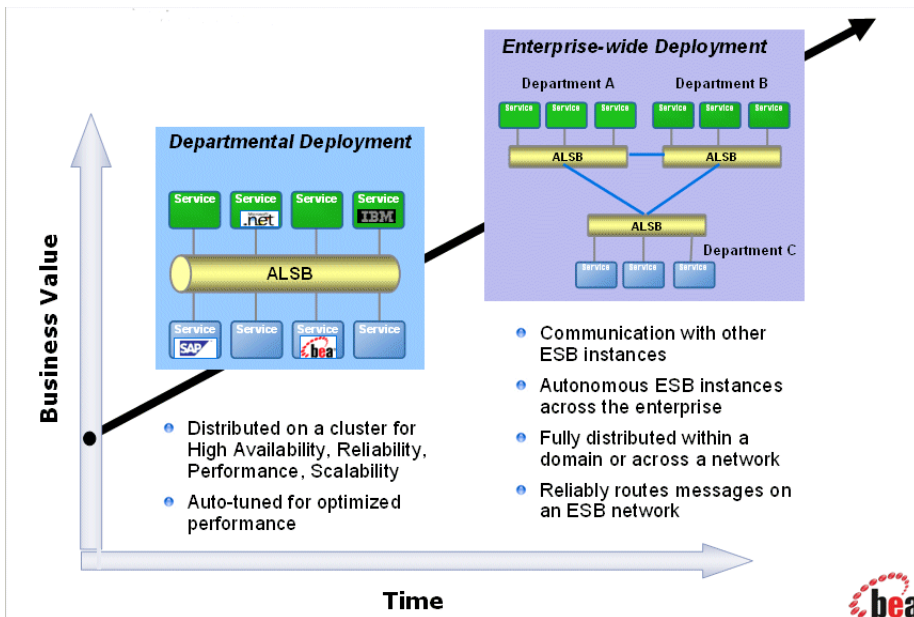
Figure 2-6 AquaLogic Service Bus Deployments
