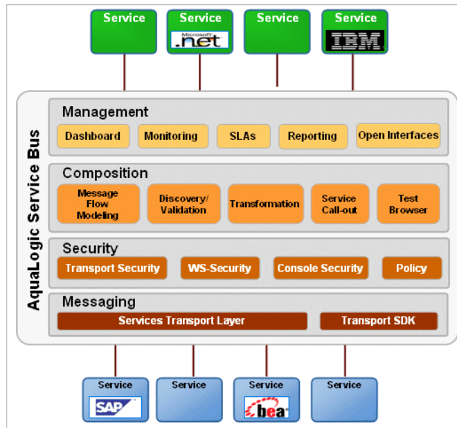
Figure 1-8 AquaLogic Service Bus Functional Features
