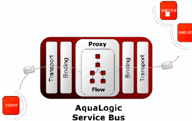
Figure 2-3 Binding and Transport Layers in AquaLogic Service Bus
