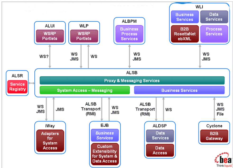
Figure 1-6 AquaLogic Service Bus Shared Services Product Architecture
