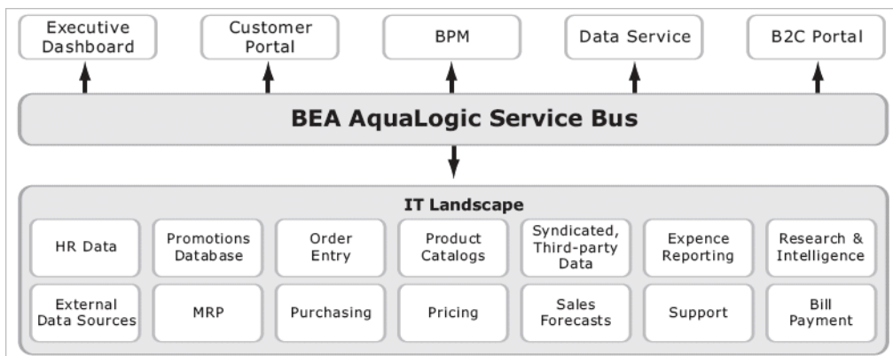
Figure 1-7 AquaLogic Service Bus Intermediary
