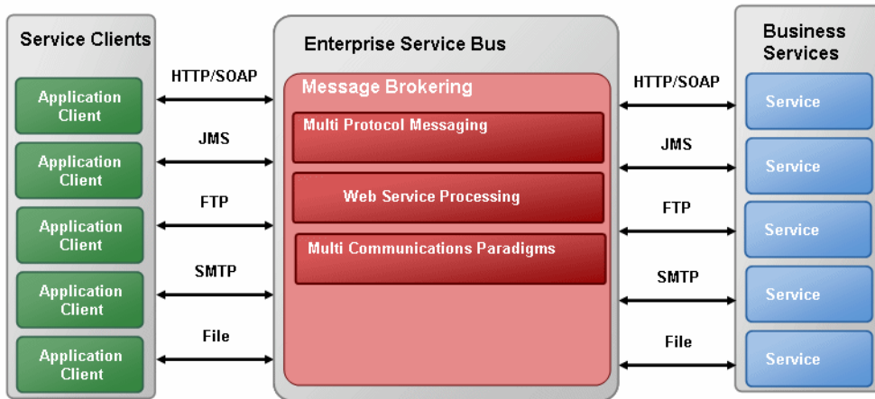
Figure 3-1 Message Brokering in AquaLogic Service Bus
