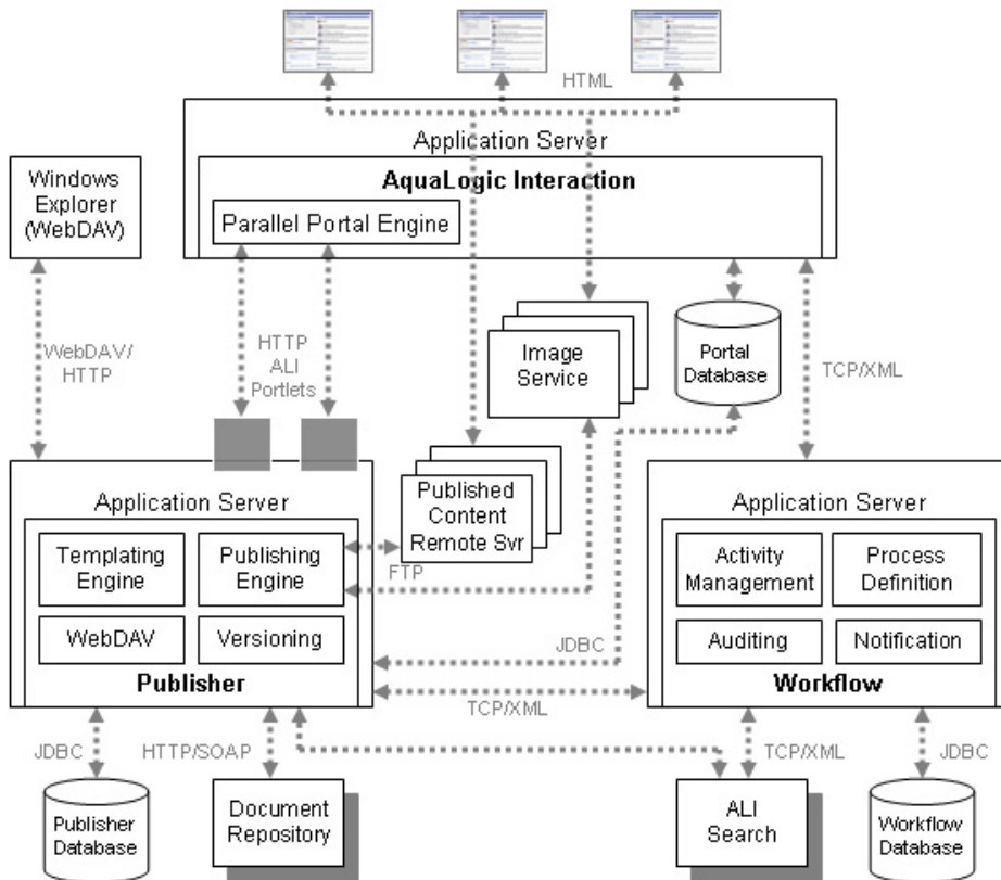
Figure 2-1 Publisher Architecture
