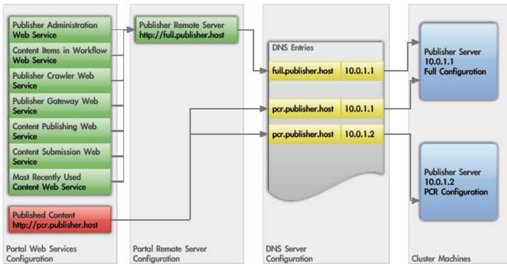
Figure C-1 High-Availability Published Content Configuration
