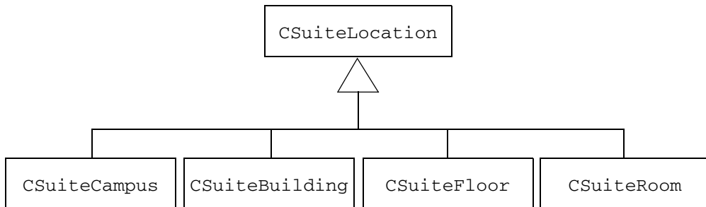
Figure 2-1 Location Class Hierarchy
