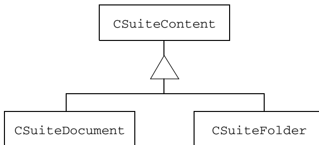
Figure 2-2 Content Class Hierarchy
