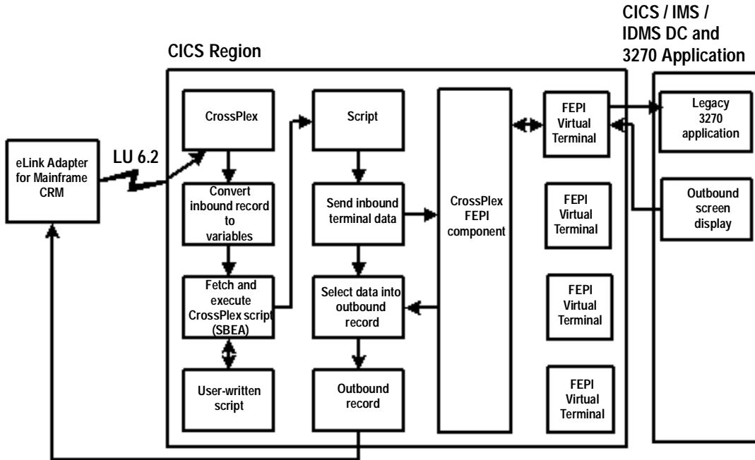
Figure 7-1 CrossPlex Architecture
