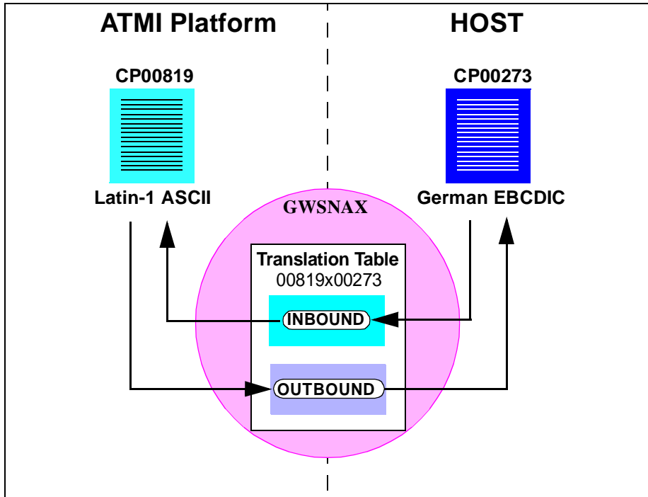
Figure 5-1 eLink Adapter for Mainframe Code Page Translation
