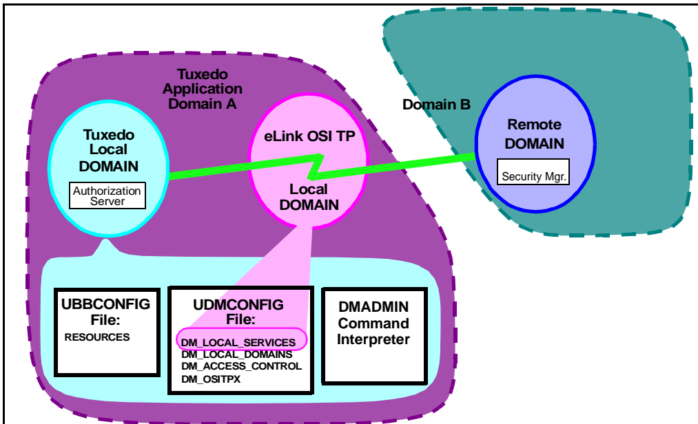
Figure 4-2 eLink OSI TP Security Elements
