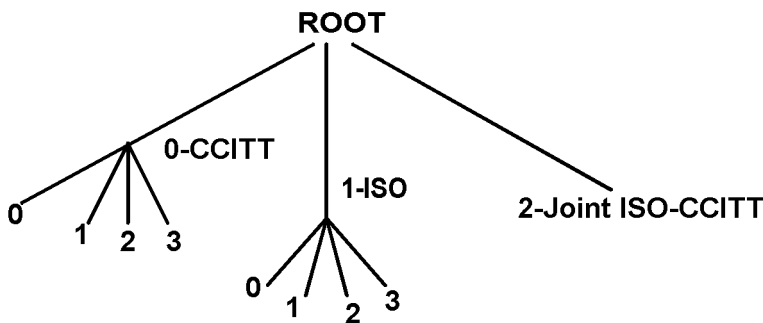
Figure 3-1 Example of an Application Entity Title
