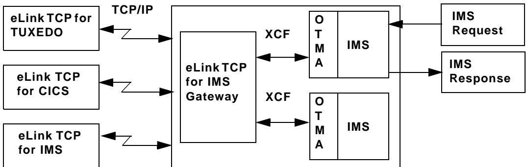
Figure 2-1 IMS Processing
