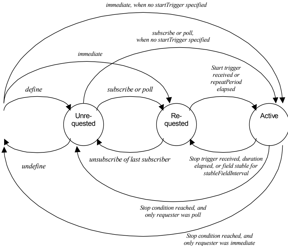
Figure 5-1 State Diagram
