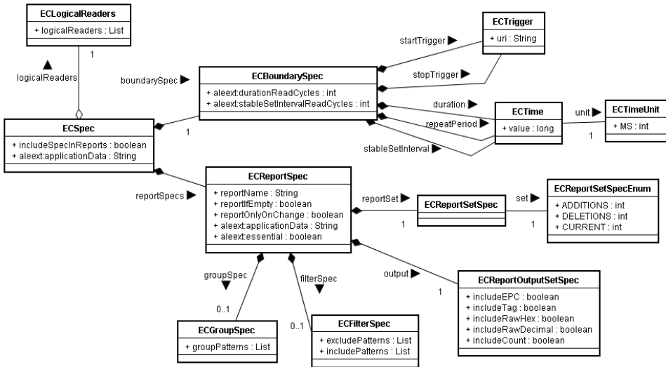
Figure 5-2 ECSpec UML Diagram
