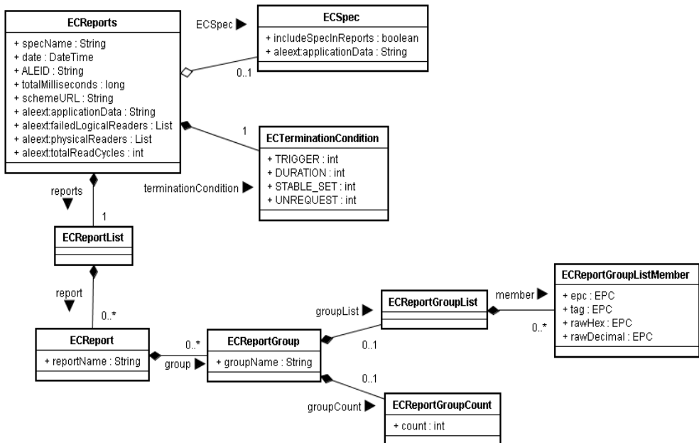
Figure 5-3 ECReports UML Diagram
