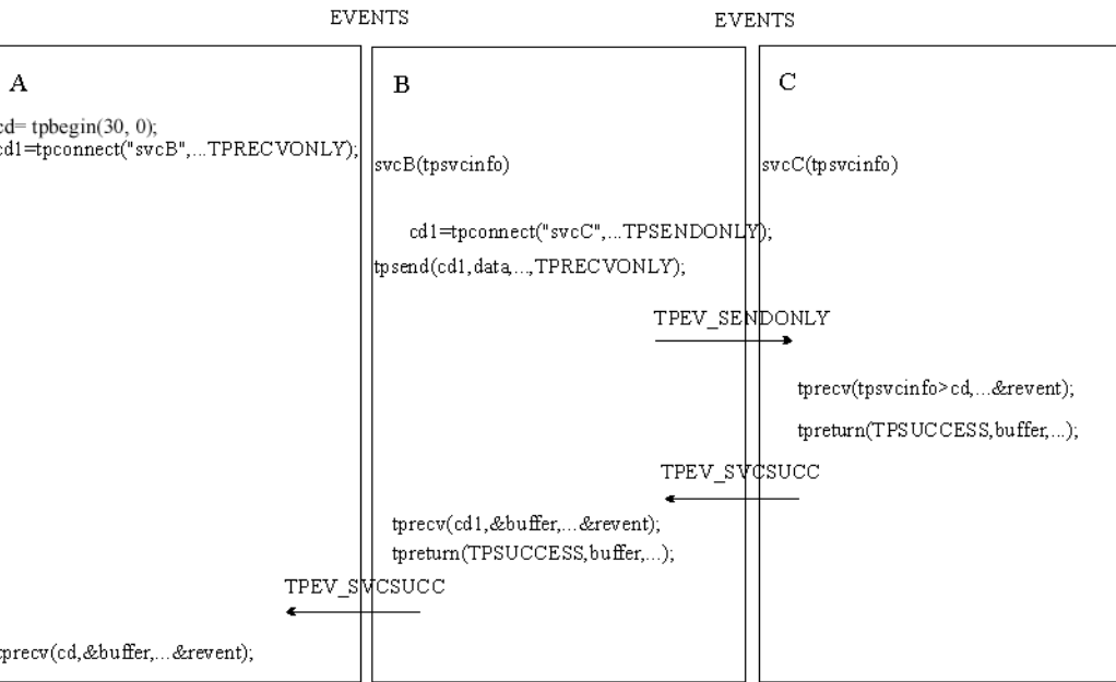
Figure 9-1 Connection Hierarchy in Transaction Mode
