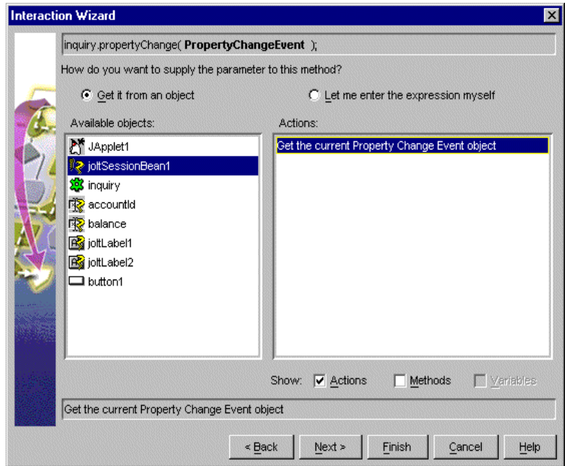
Figure 6-17 Select joltSessionBean1
