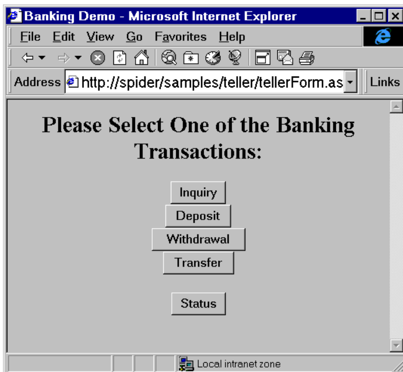
Figure 8-2 tellerForm.asp Example
