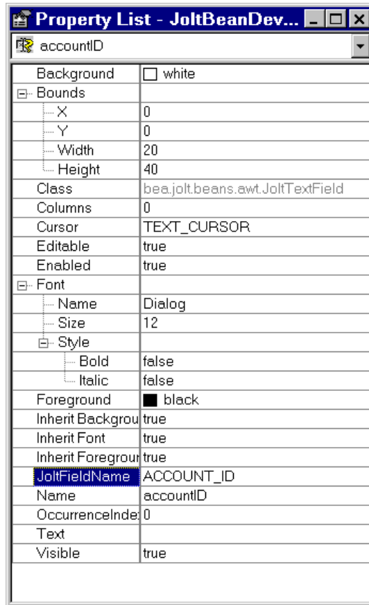
Figure 6-8 Revised JoltFieldName in the JoltTextField Property List
