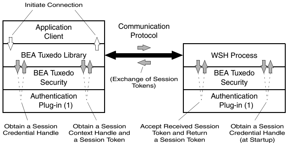
Figure 1-3 Client-WSH Authentication
