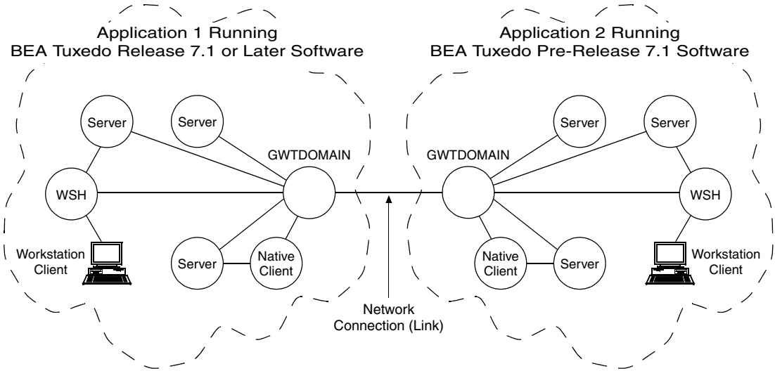
Figure 1-11 Inter-Domain Interoperability
