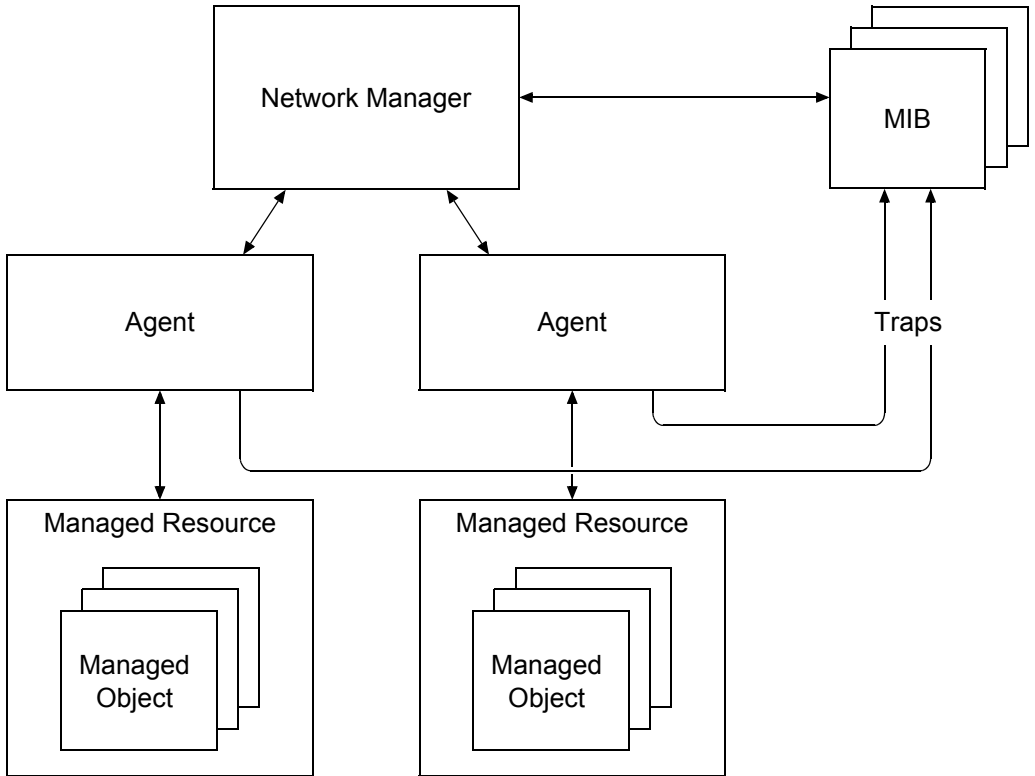
Figure 1-2 Manager/Agent Model
