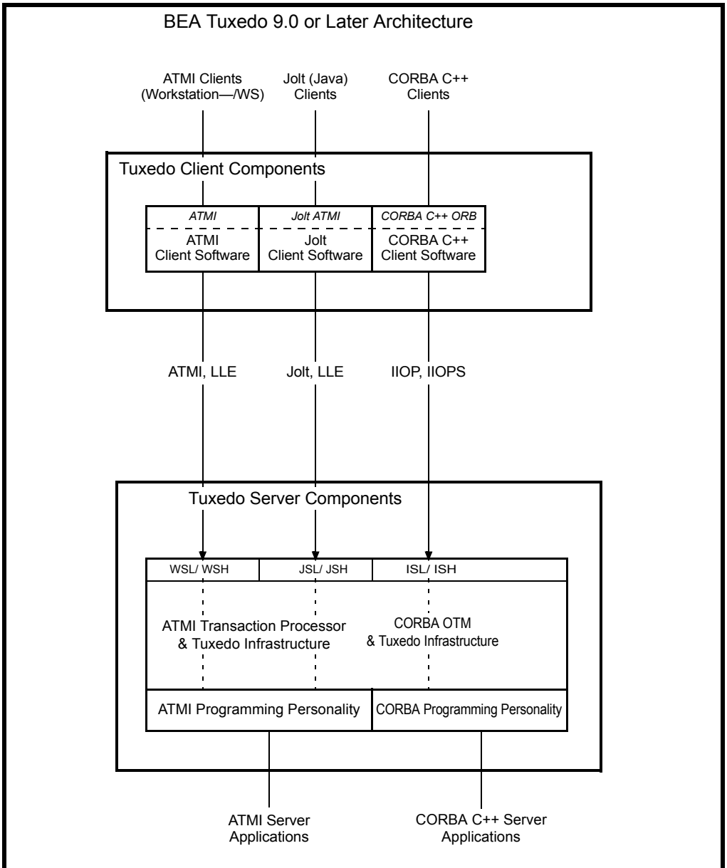
Figure 1-4 BEA Tuxedo Client and Server Components
