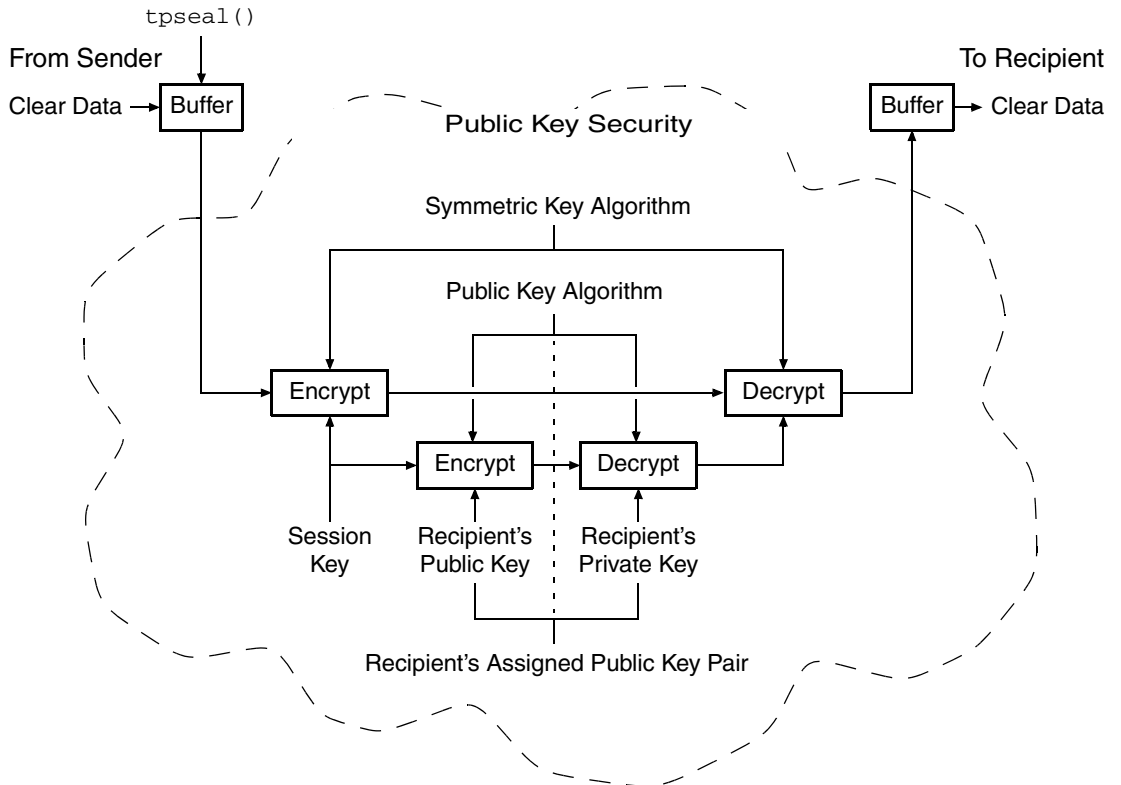
Figure 1-9 ATMI PKCS-7 End-to-End Encryption
