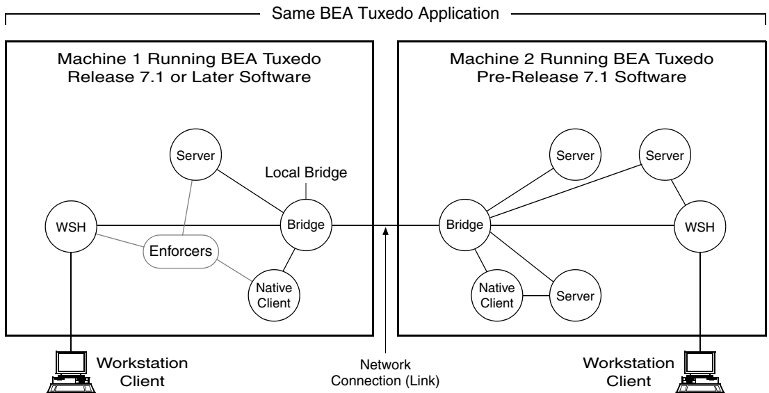
Figure 1-13 Enforcing Intra-Domain Interoperability Rules for Public Key Security
