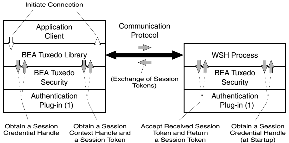
Figure 1-3 Client-WSH Authentication
