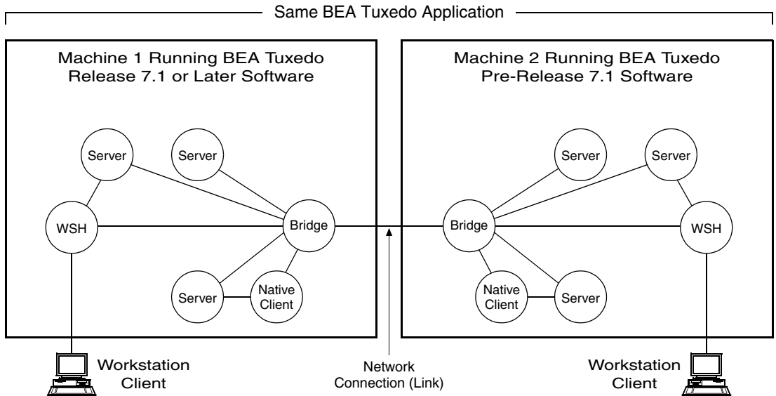
Figure 1-12 Intra-Domain Interoperability
