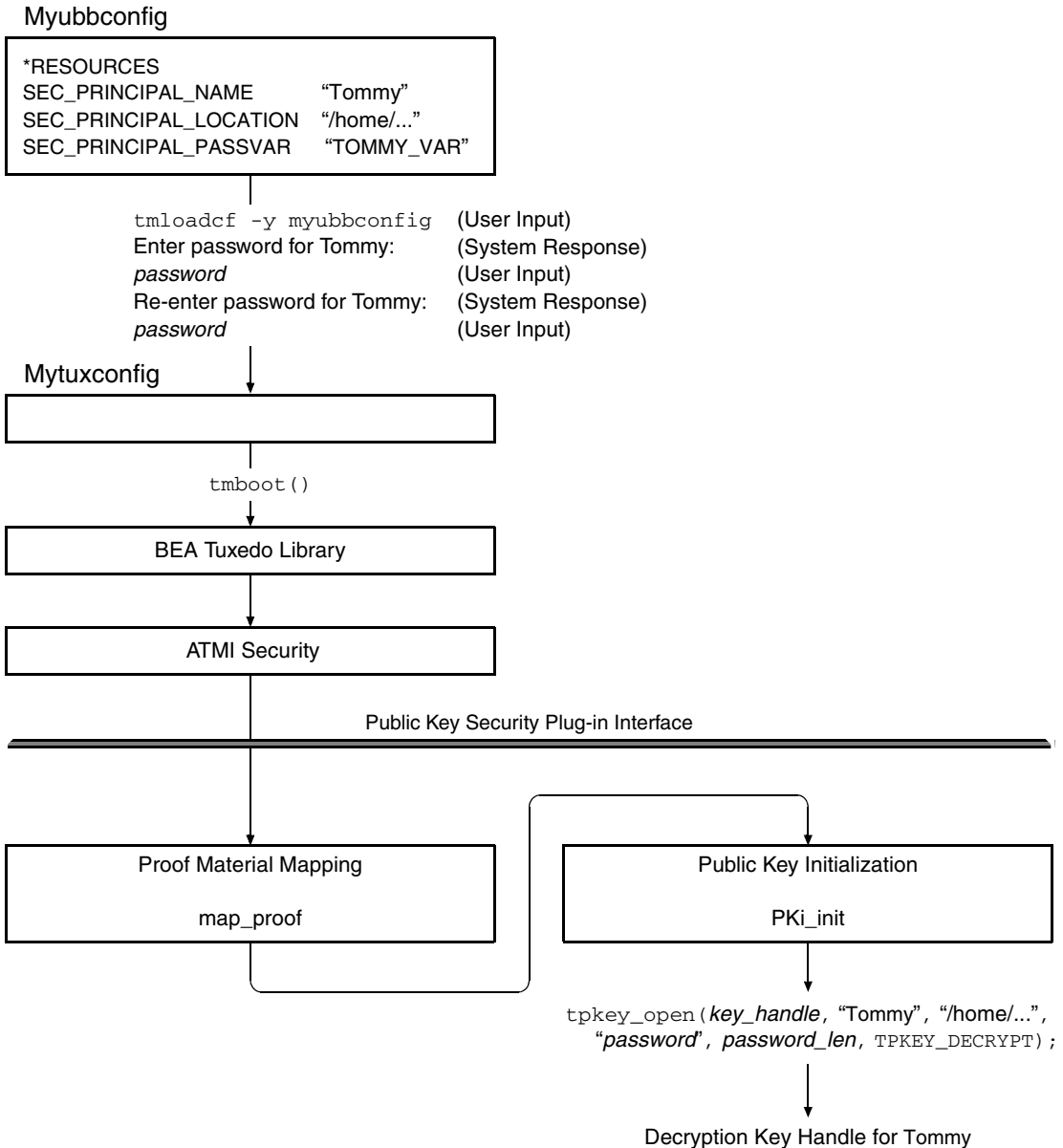
Figure 2-13 How a Decryption Key Is Initialized Example
