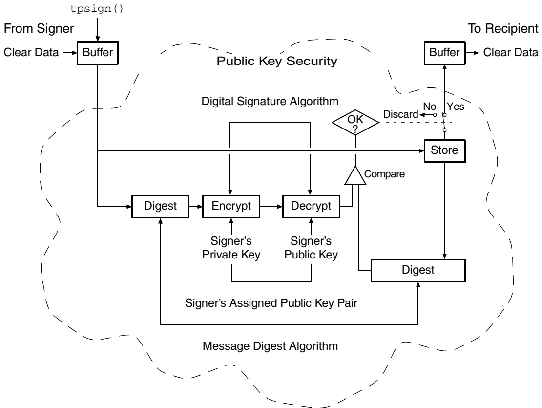
Figure 1-7 ATMI PKCS-7 End-to-End Digital Signing
