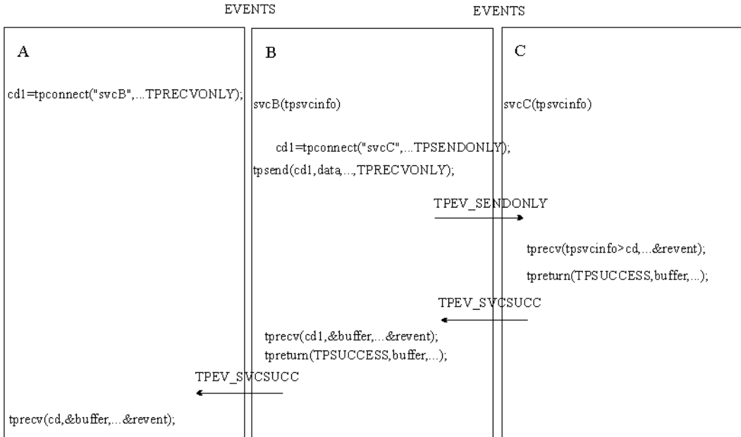
Figure 7-3 Connection Hierarchy
