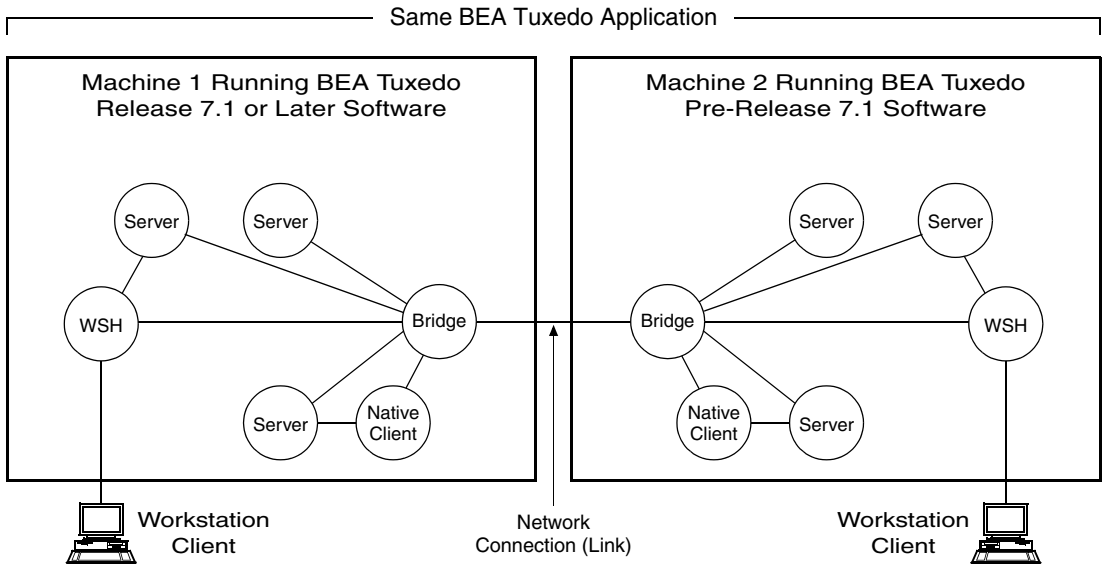
Figure 1-12 Intra-Domain Interoperability
