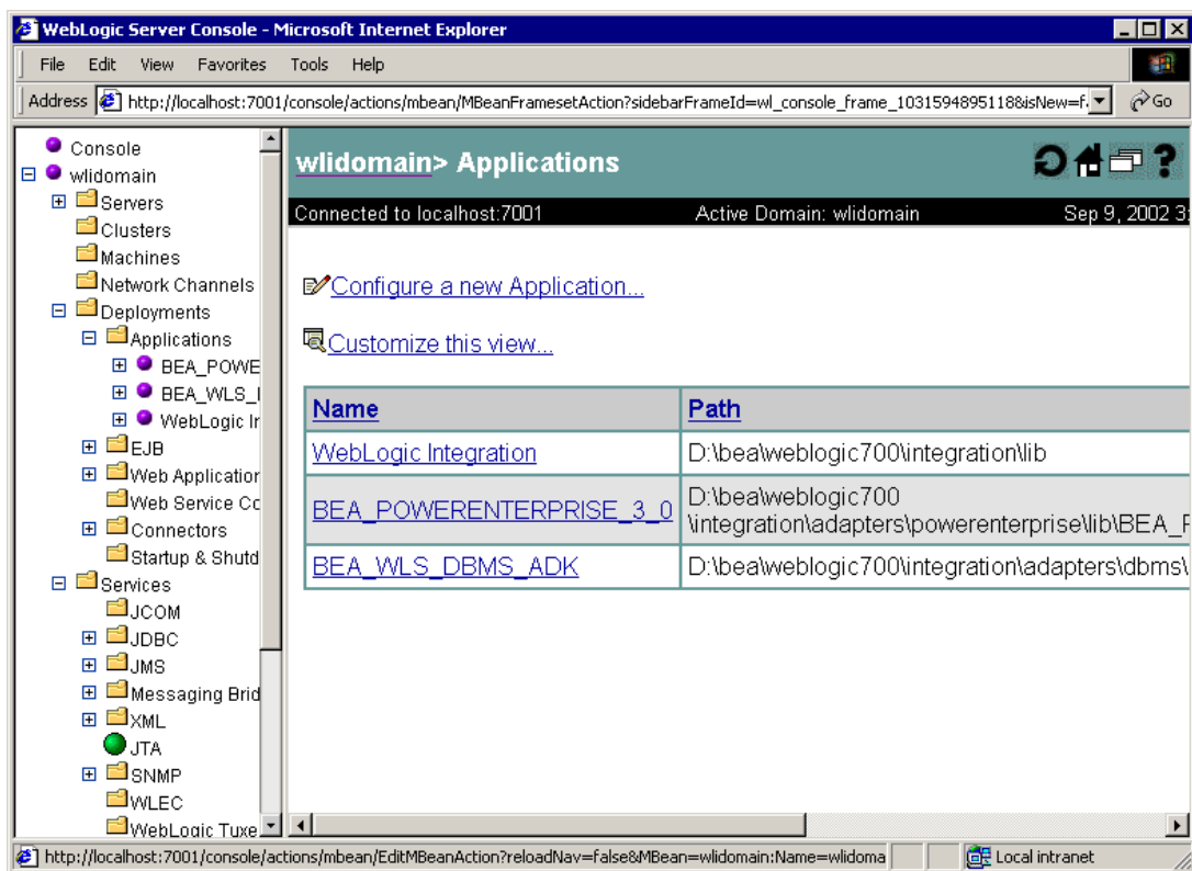
Figure 1-2 Applications Window
