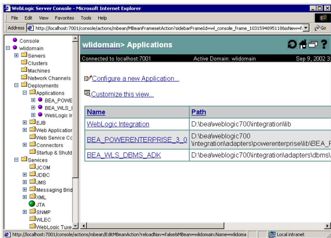
Figure 1-2 Applications Window
