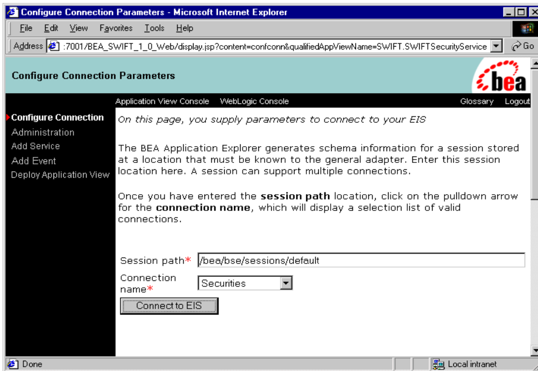
Figure 3-3 Configure Connection Parameters
