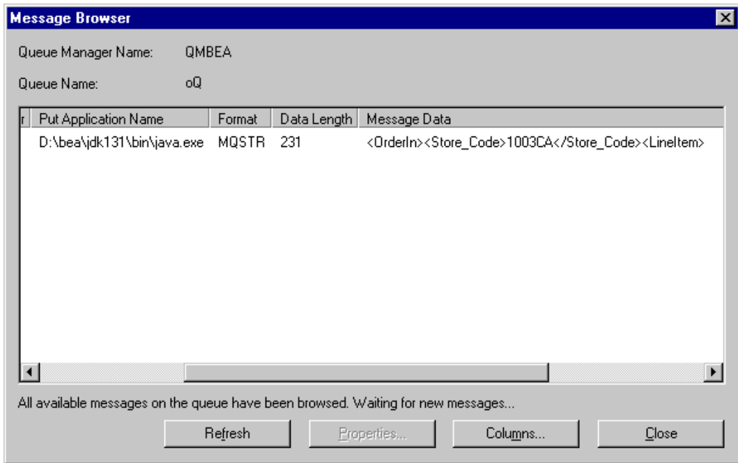
Figure 3-15 Message Browser Window
