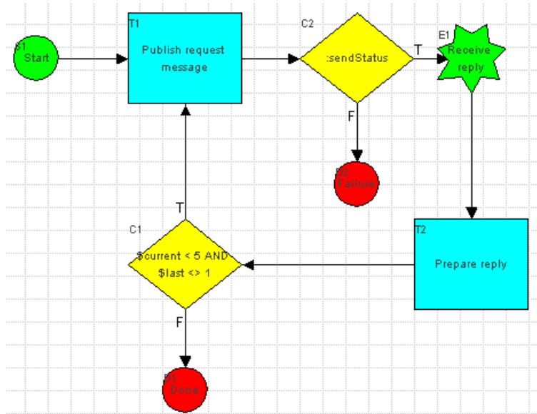
Figure 3-12 The wlpiverifier_init Workflow
