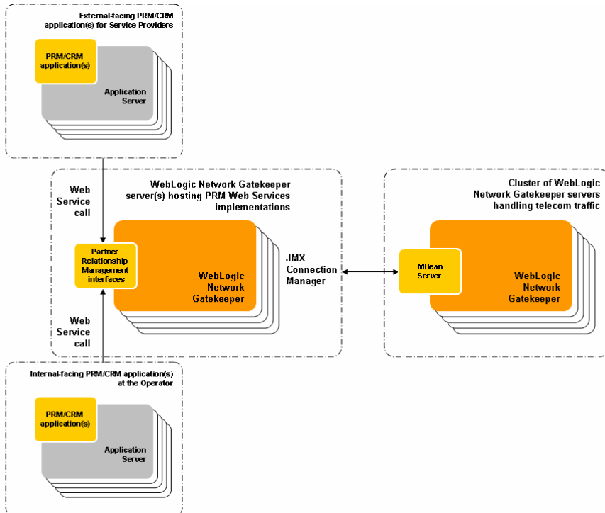
Figure 2-1 Deployment example
