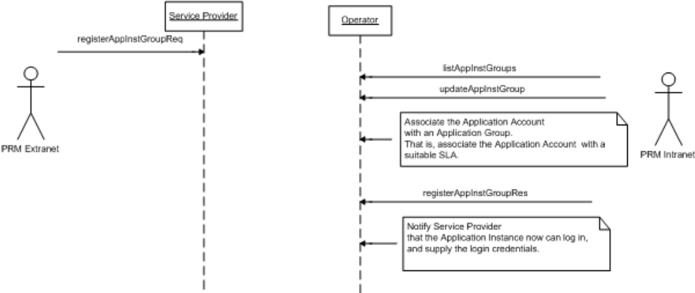
Figure 5-3 Registering a new Application Instance
