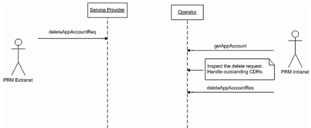
Figure 5-7 Service provider requests an account deletion
