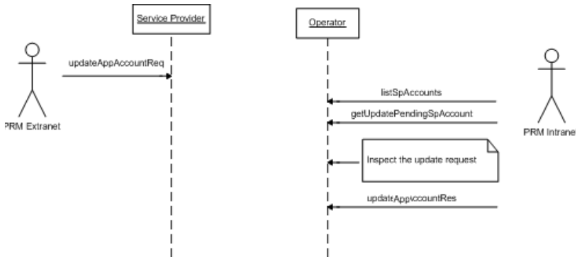
Figure 5-6 Service Provider requests an account update
