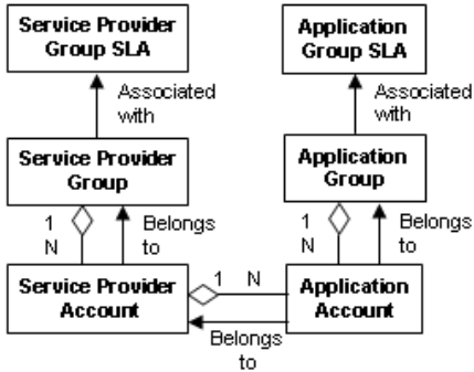
Figure 3-1 Partner Management Model
