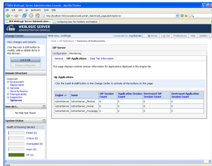
Figure 3-5 Application Metrics
