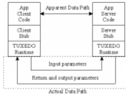
Figure 1-1 RPC Communication
