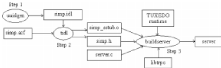
Figure 1-2 Building an RPC Server
