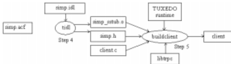
Figure 1-3 Building an RPC Client
