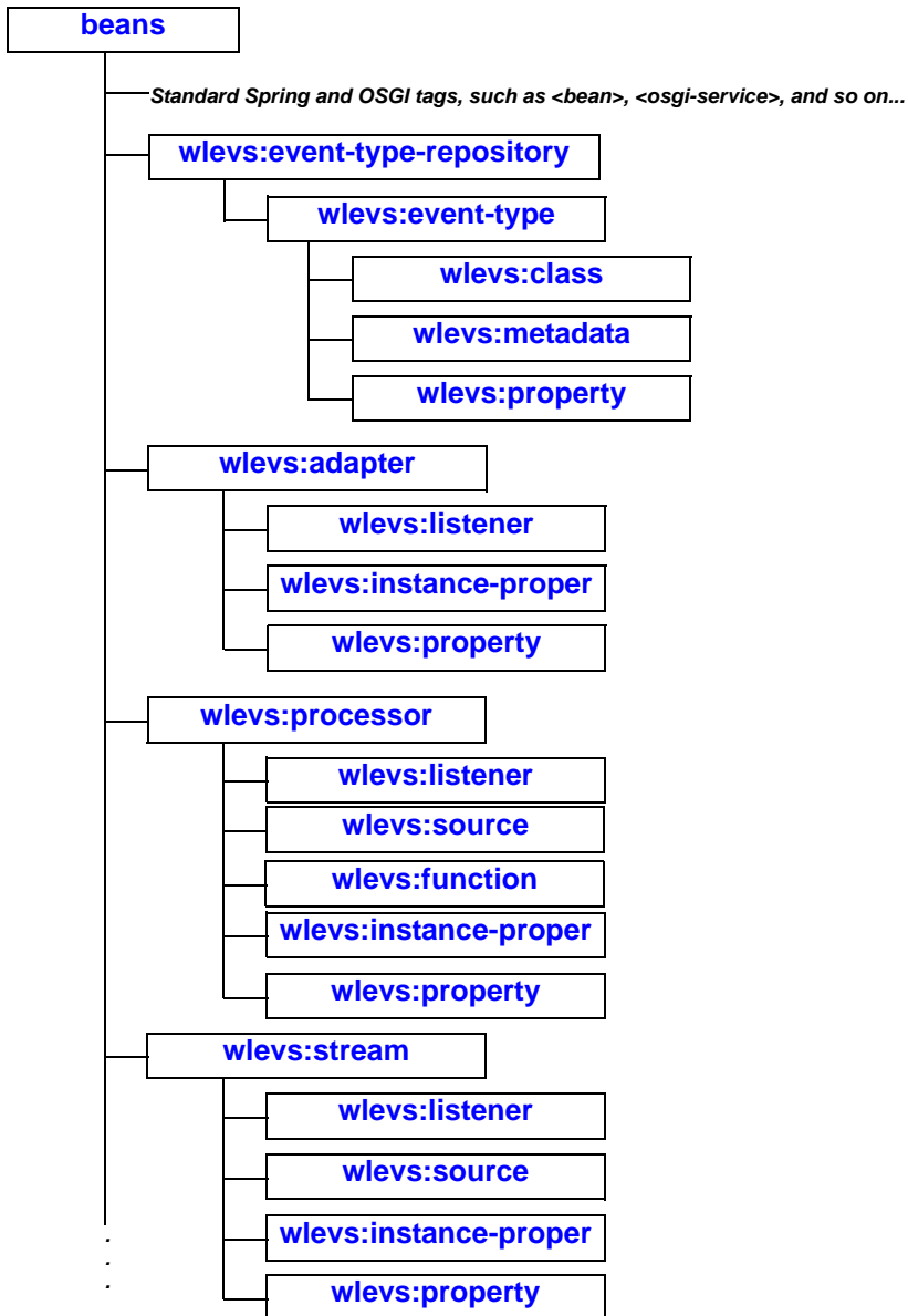
Figure 2-1 Hierarchy of Oracle CEP Spring Tags
