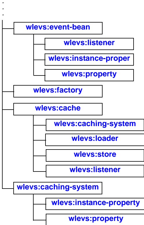
Figure 2-2 Hierarchy of Oracle CEP Spring Tags (continued)
