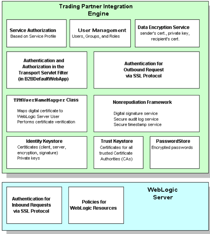
Figure 4-1 WebLogic Security Model for Trading Partner Integration
