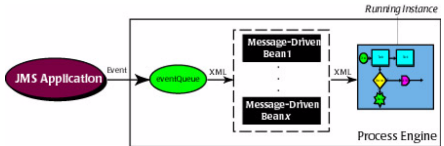
Figure 6-1 Overview of JMS
