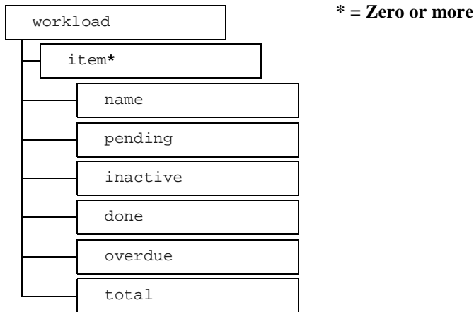
Figure A-18 Workload Response DTD Hierarchy Diagram
