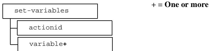
Figure A-10 Client Set Variables Request DTD Hierarchy Diagram
