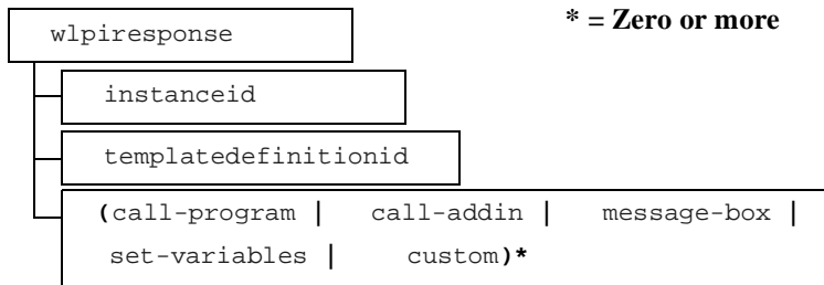
Figure A-9 Client Request DTD Hierarchy Diagram
