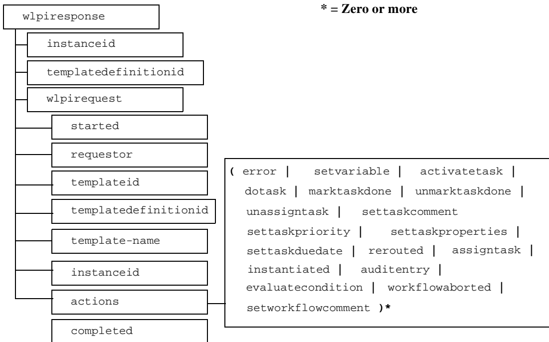
Figure A-1 Audit DTD Hierarchy Diagram
