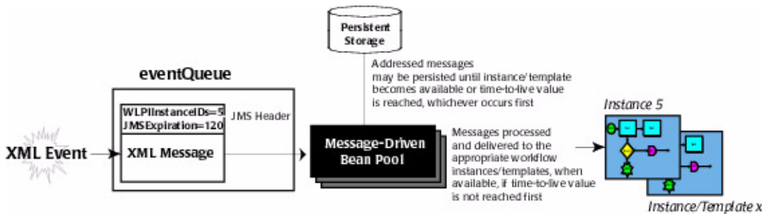
Figure 6-2 Guaranteed Message Delivery
