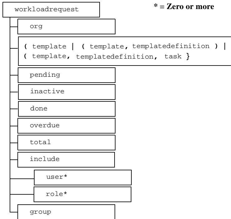
Figure A-17 Workload Request DTD Hierarchy Diagram
