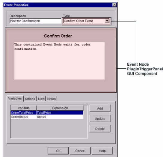
Figure 4-6 PluginTriggerPanel GUI Component for a Event Node
