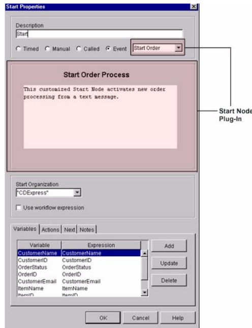
Figure 1-1 Plug-In Example: Start Node
