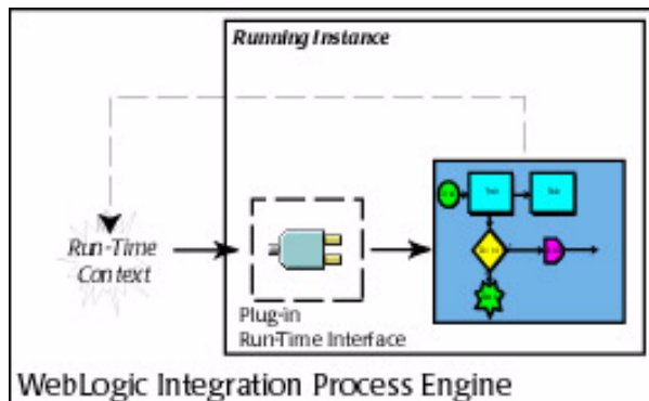
Figure 4-10 Context Passing
