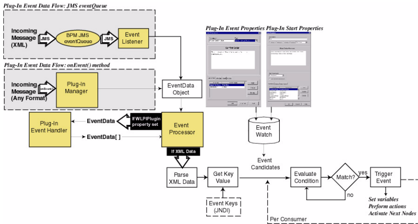
Figure 6-1 Plug-In Event Data Flow
