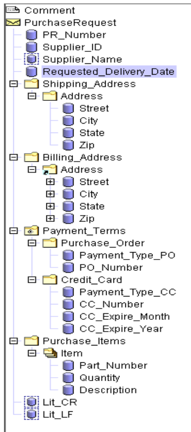
Figure C-2 Completed Navigation Tree for Purchase Order Sample
