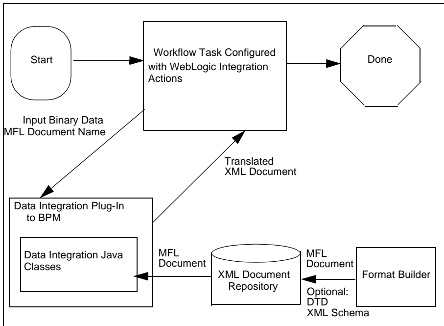
Figure 1-5 Data Integration and BPM Relationship
