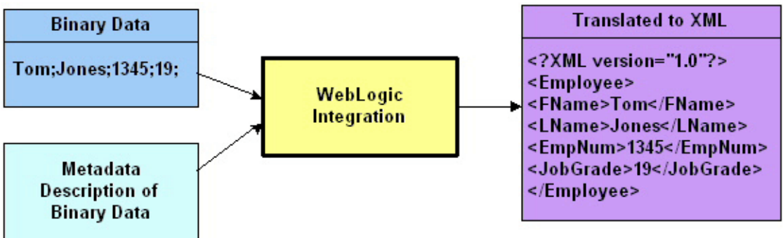
Figure 1-1 XML Data Translation of: Tom;Jones;1345;19;
