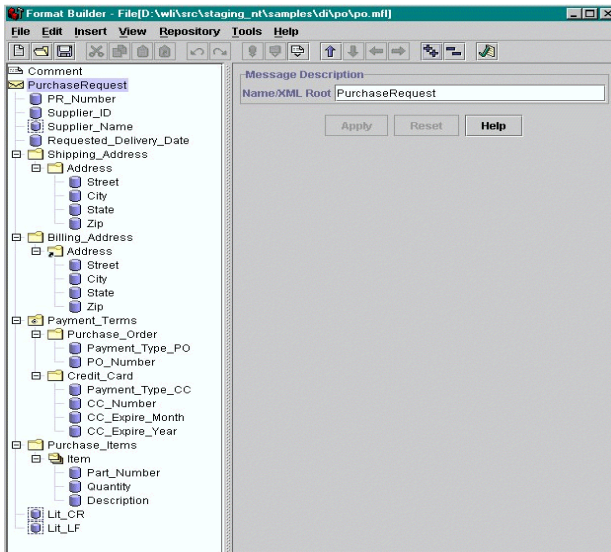
Figure 2-1 Format Builder Main Window
