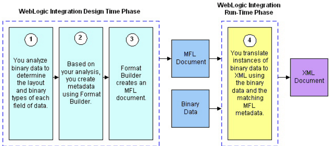
Figure 1-2 Event Flow for Translating Data
