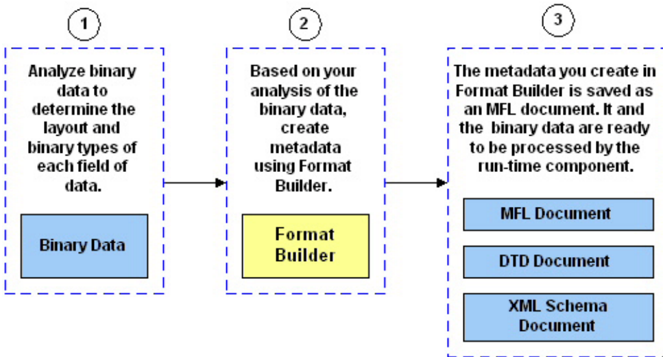
Figure 1-3 Design Time Process Flow Through Format Builder
