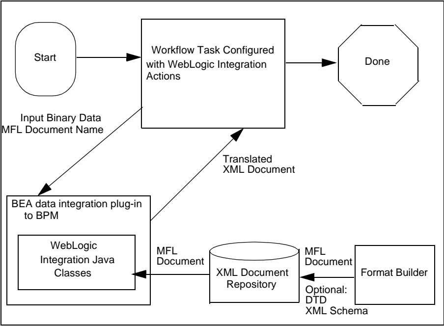
Figure 6-1 Run-Time Plug-In to BPM
