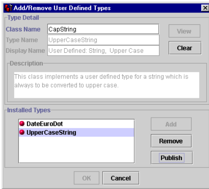
Figure B-2 Add/Remove User Defined Types Dialog Box
