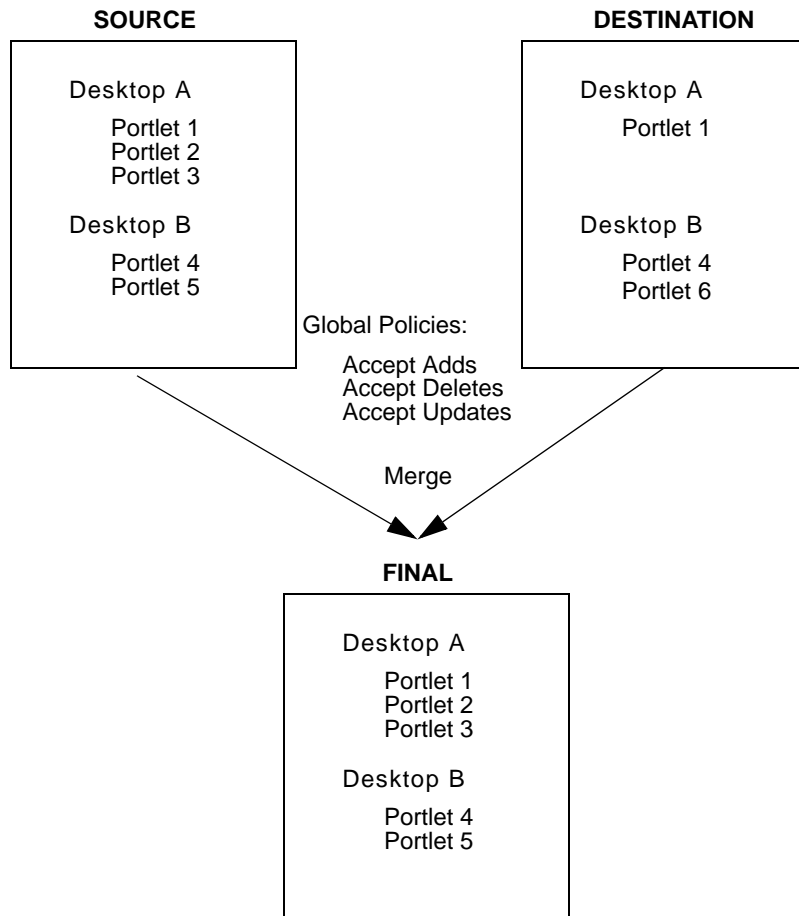
Figure 6-9 Accepting Adds and Deletes
