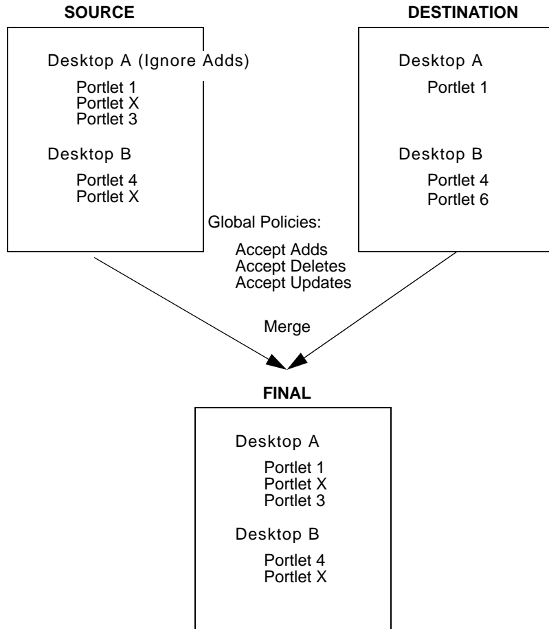
Figure 6-12 Local Policies and Library Instances
