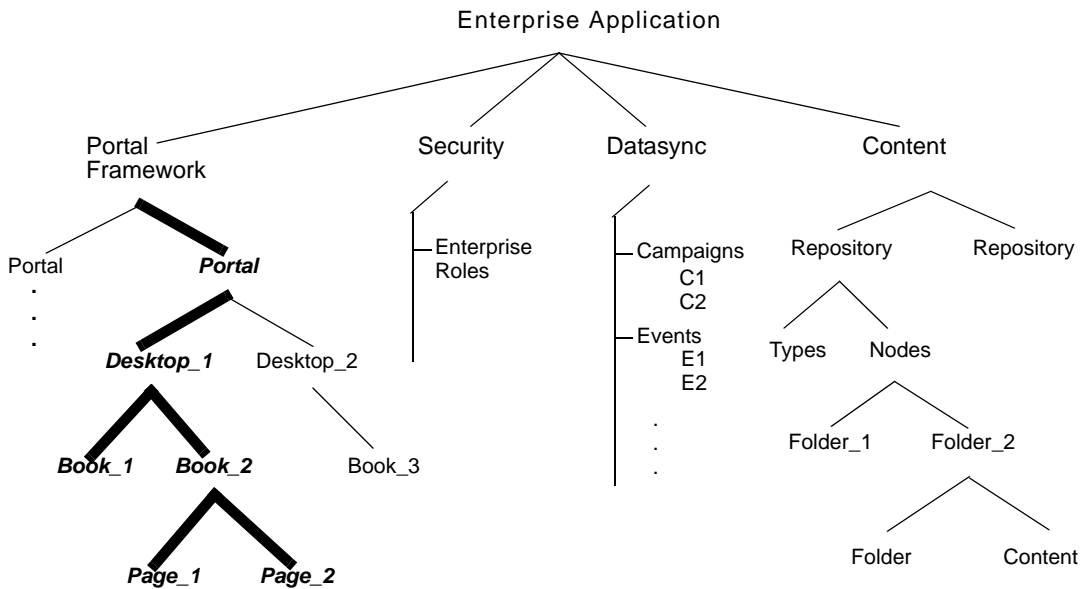
Figure 6-6 Scoping to Desktop_1
