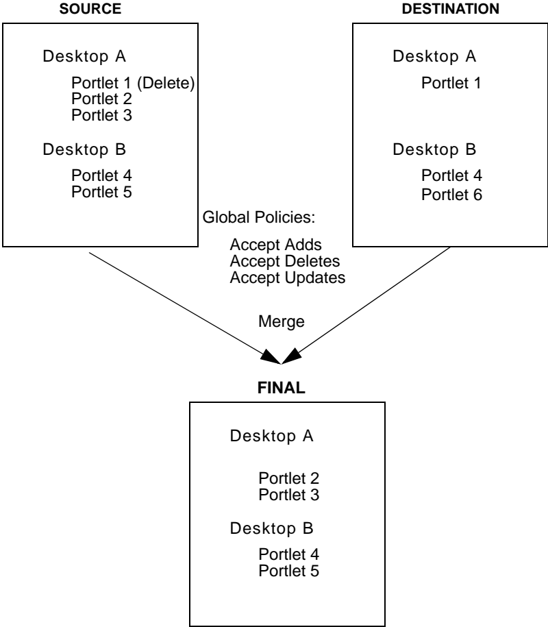
Figure 6-11 Local Policy Overrides Global Policy
